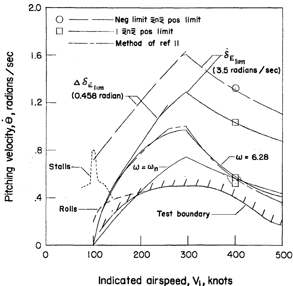
Figure 11.- Comparison of test results with maximum calculated pitching velocities obtained by maneuvering the F-86A airplane sinusoidally within the V-n diagram at sea level. (Symbols at 400 knots are for altitude of 20,000 feet.)
