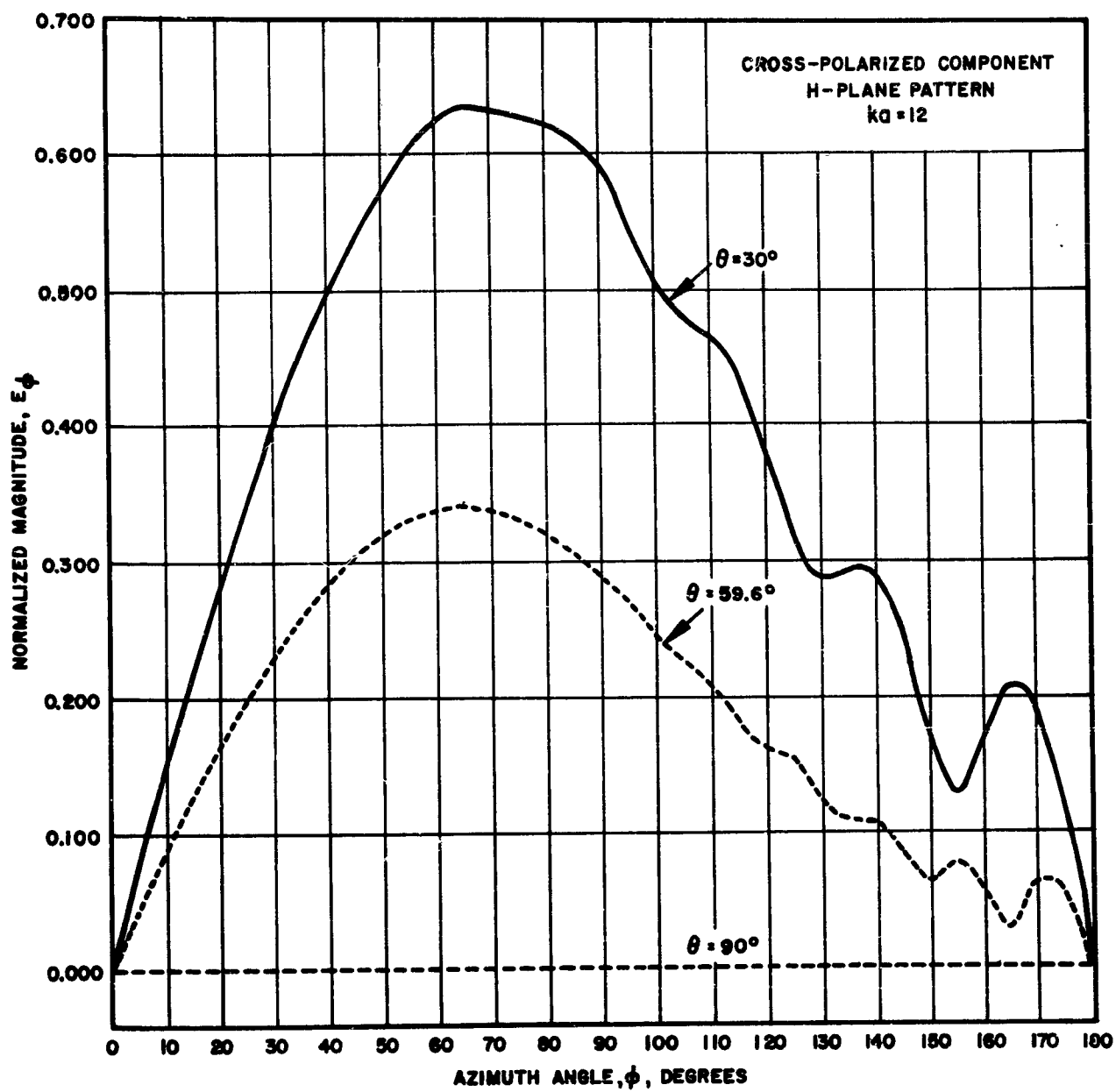
Figure II-10. Cross-Polarized Component of H-Plane Pattern for Circumferential Half-Wave Length Slot
