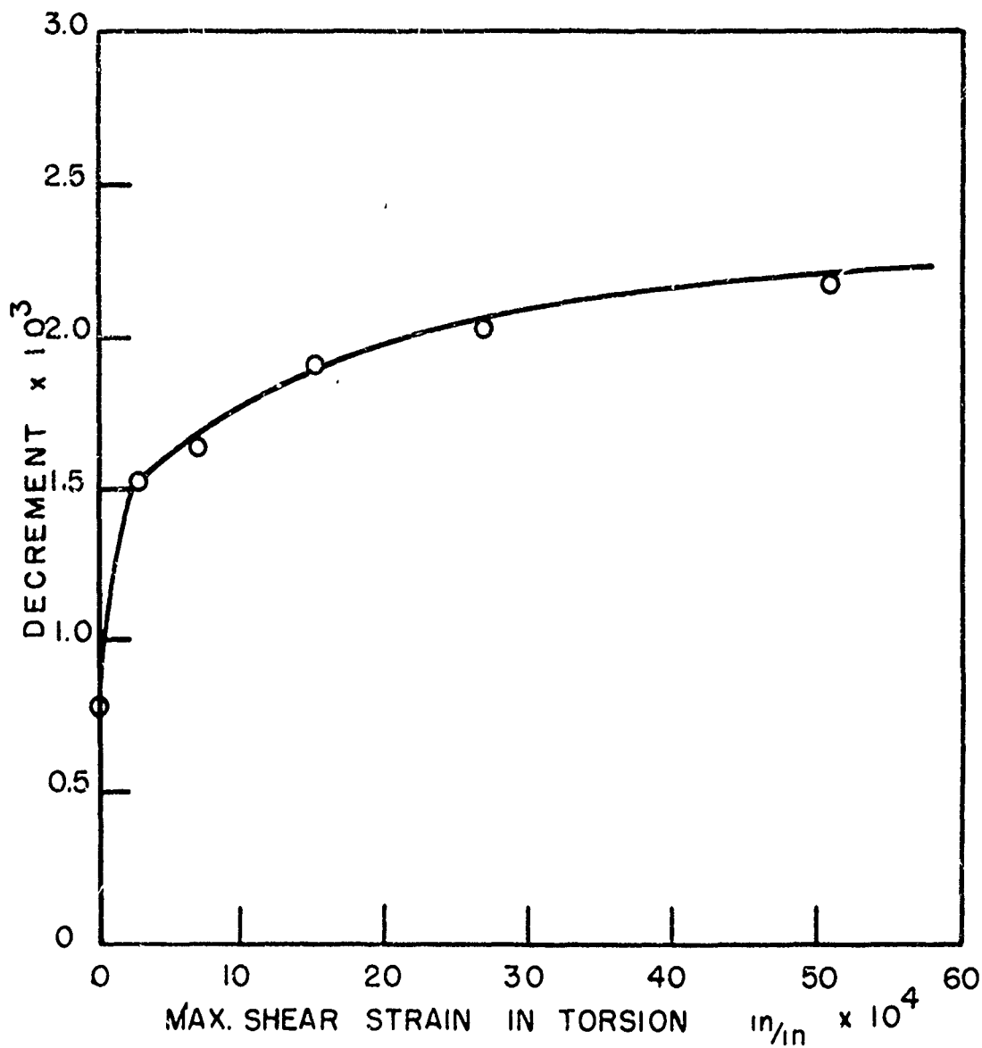
FIG. 8 EFFECT OF TORSIONAL STRAIN ON INTERNAL FRICTION Ag 2 MAXIMUM STRAIN AMPLITUDE 1 \times 10^{-7} \text{ in/in}
