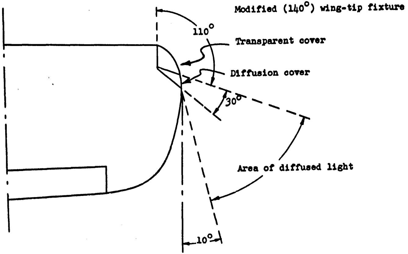
FIGURE 2. Recommended alternative methods for wing-tip formation lighting.
