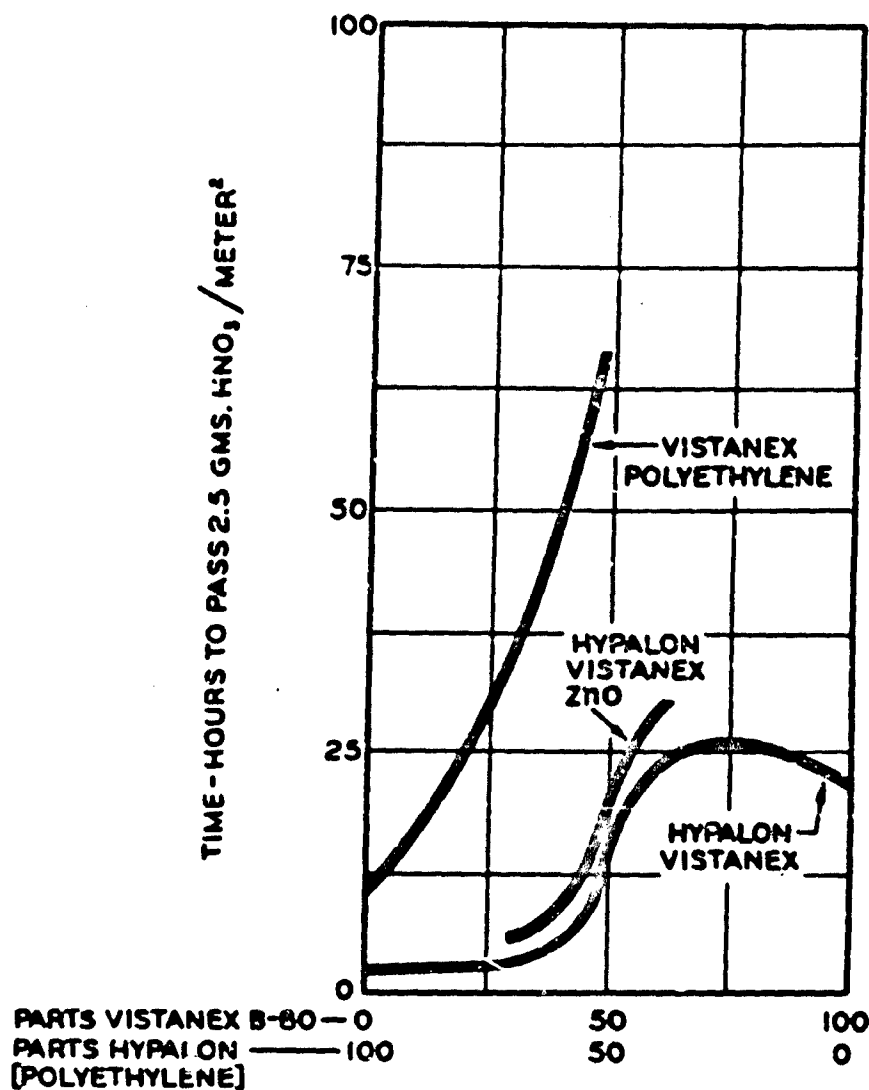
FIG. II - THE EFFECT OF BLEND COMPOSITION ON THE NITRIC ACID PERMEABILITY OF PRESS MOLDED HYPALON-VISTANEX B-80 FILMS-.008"
