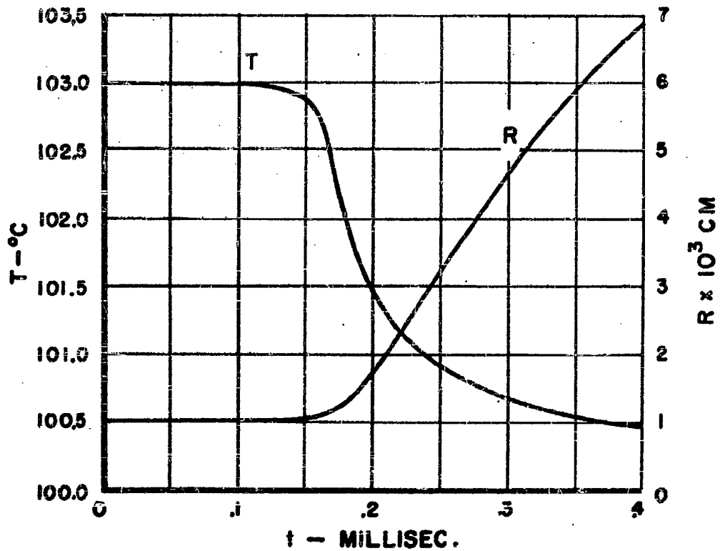
Fig. 8 - Theoretical radius and bubble wall temperature curves for the 103^\circ vapor bubble of Fig. 7.
