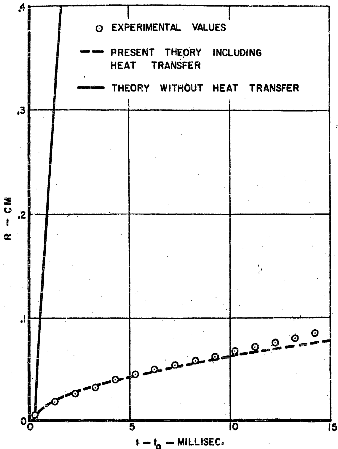
Fig. 4 - Comparison of theoretical bubble radius-time values with experimental values for water at 1 atm. external pressure, superheated to 103.1^{\circ}\text{C} . The solid curve is the Rayleigh growth curve, obtained by neglecting heat transfer effects; the dashed curve is that predicted by the asymptotic solution of the text, which takes heat transfer into account.
