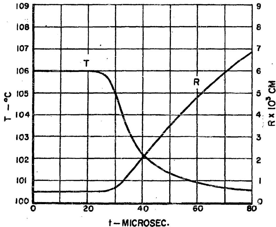
Fig. 10 - Theoretical radius and bubble wall temperature curves for the 106°C vapor bubble of Fig. 9.
