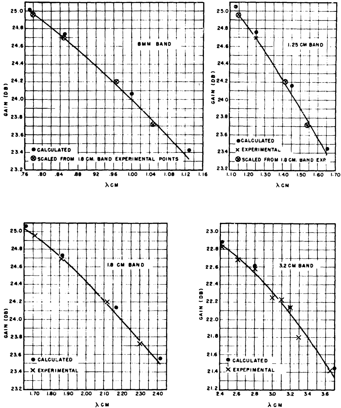
Fig. A-5 (a). Gain curves
