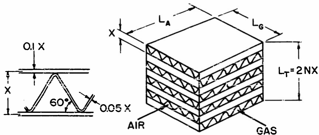
(a) PLATE-FIN SURFACE
