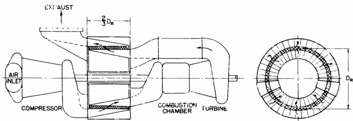
(a) PLANT LAYOUT
