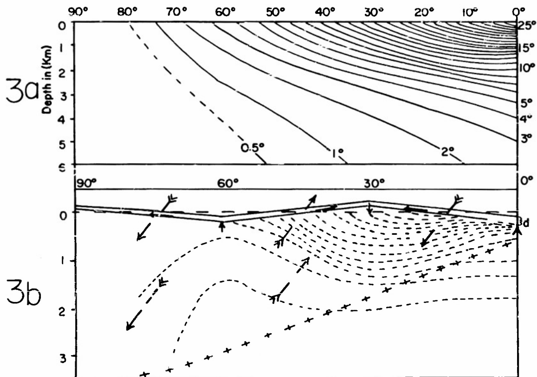
Fig. 3a. Computed temperature distribution in an ocean at rest (equilibrium of heat conduction with given sea surface conditions A_y/A_z = 10^7 ).
