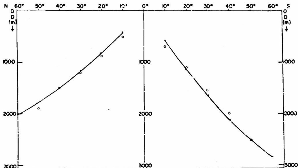
Figure 2. Average depth, D , of the layer of no motion in the Atlantic Ocean. The curves \text{---}\circ\text{---} represent D(\varphi) = \text{const.} \sin \varphi , and the values according to A. Defant (1941) are indicated by circles (O).
