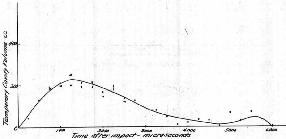
Fig. 15 - .22 cal 45 grain round nose contract bullet - 10 yd Range
