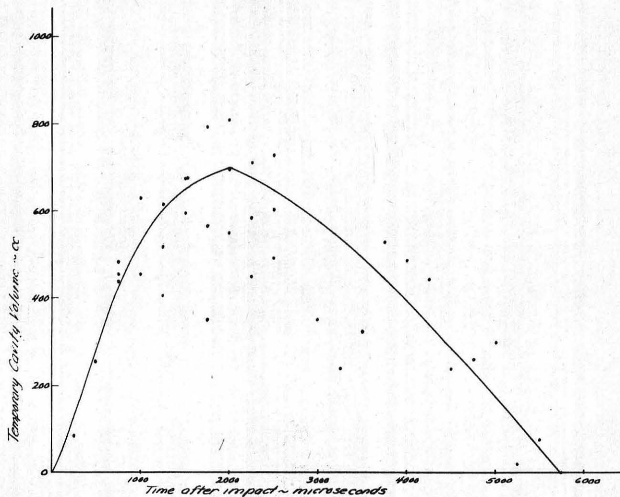
Fig. 13 - .22 cal 35 grain C2020 bullet - 10 yd Range
