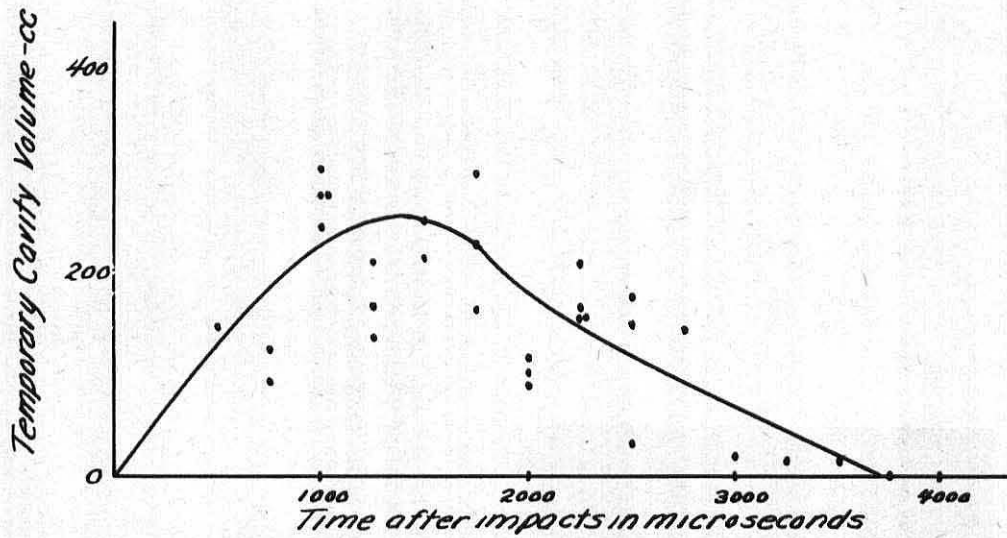
Fig. 23 - .22 cal. 35grain 62020 bullet - 100 yd Range
