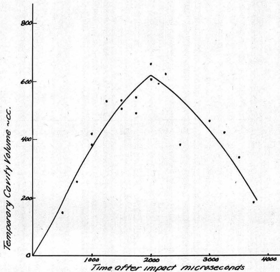
Fig. 18 - .22 cal. 45 grain soft nose Harnet bullet-75yd. Range
