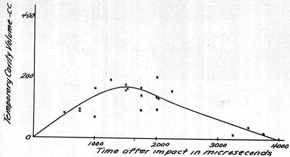
Fig. 24 - .22 cal 45grain 62021 bullet 100 yd Range
