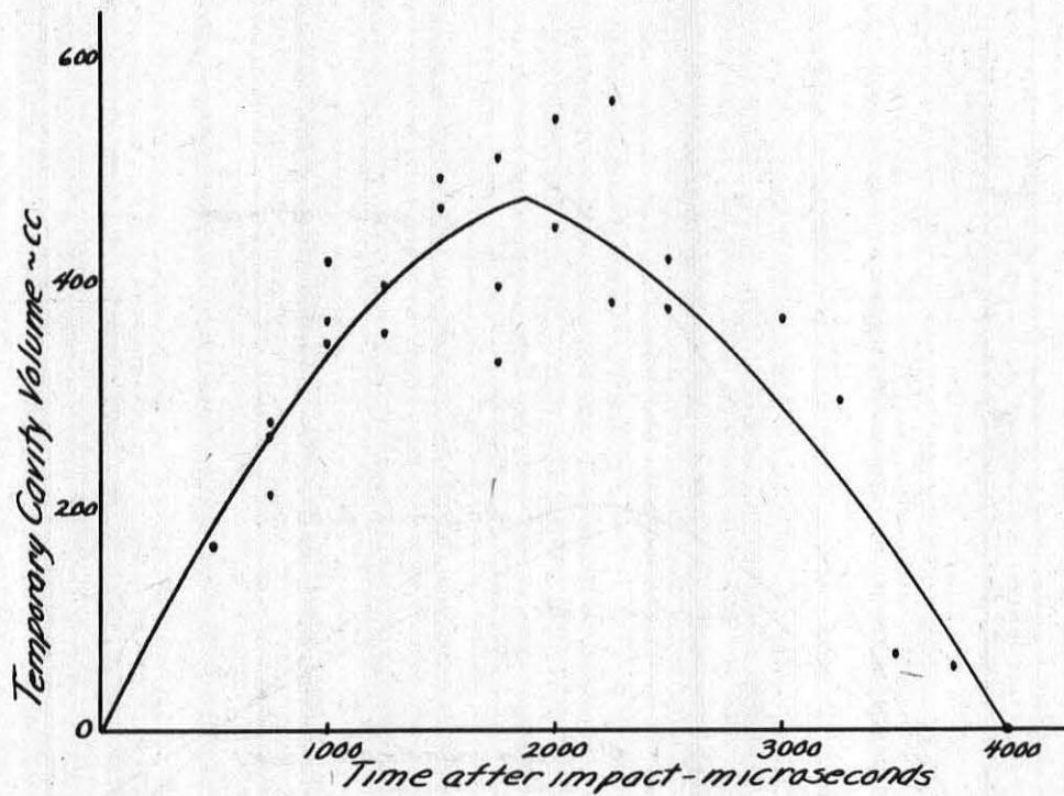
Fig. 22 - .22 cal 45 grain soft nose hornet bullet 100 Yd Range
