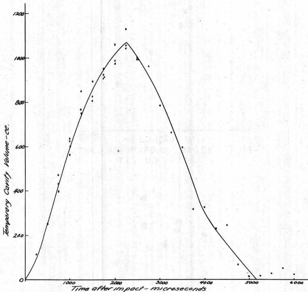
Fig. 12 - .22 cal 45 grain soft nose Harnet Bullet 10 yd Range
