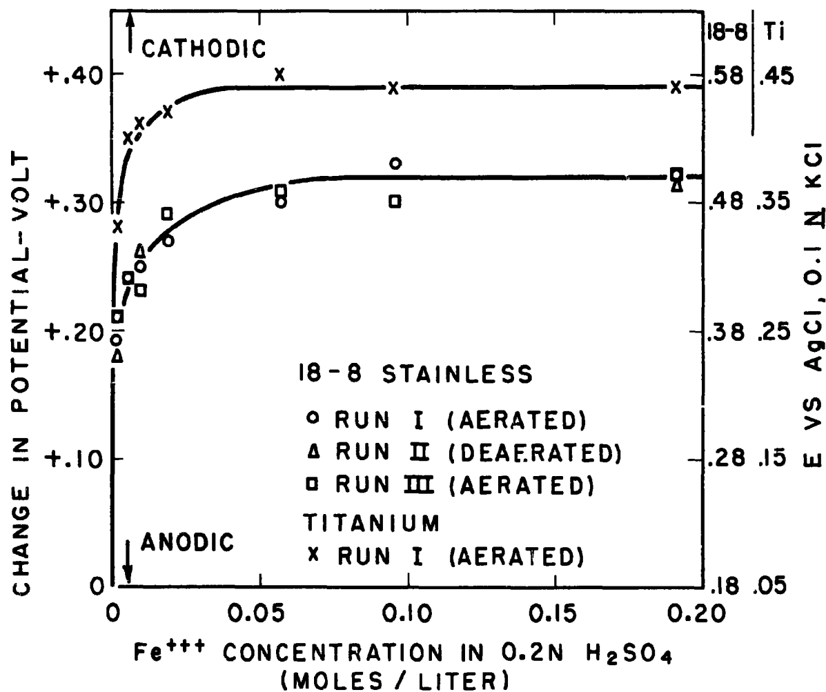
Figure 2 Effect of Fe +++ Additions on the Electrode Potentials of 18-8 Stainless Steel and Titanium in 0.2 N H 2 SO 4 . T = 25.0 ± 0.2°C.
