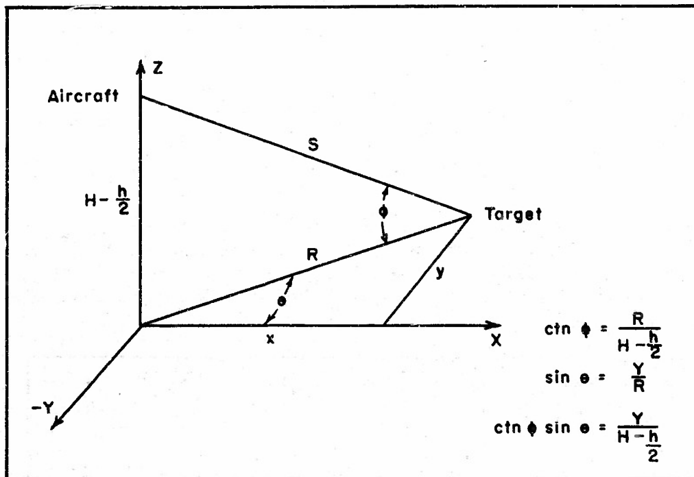
Fig. 12. Relation between vertical and horizontal angles (radar presentations).
