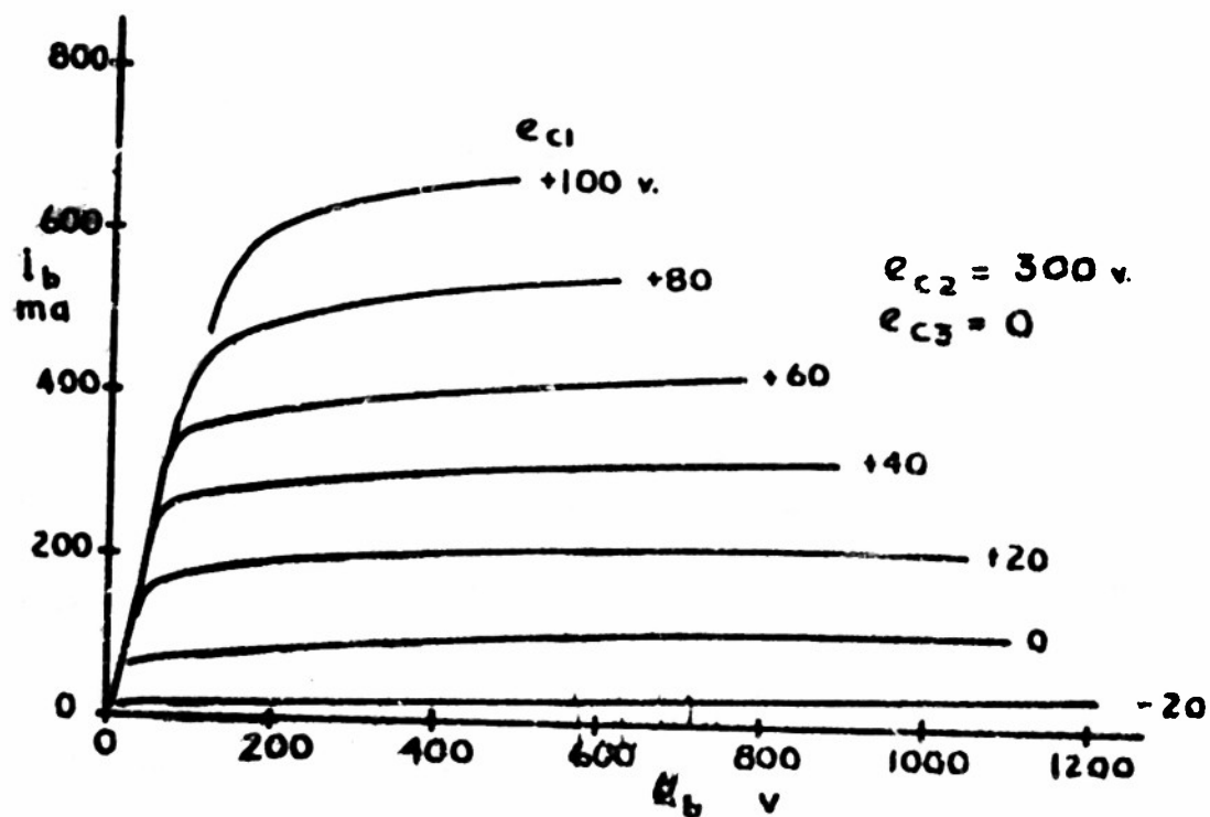
Fig. 1. Static curves for Type 814 tube
