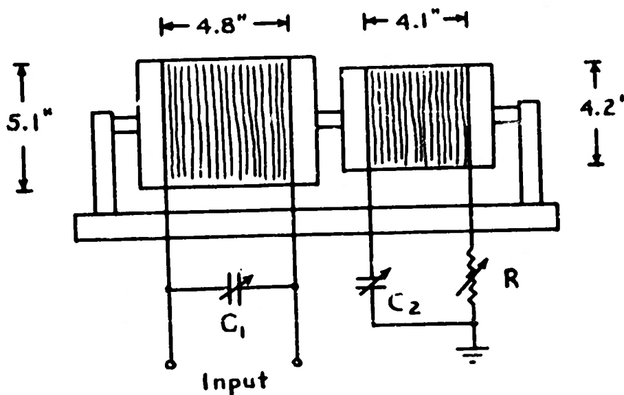
Fig. 5. Adjustable-impedance load circuit
