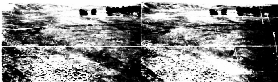
Ground Photos 30-A and 30-B. Stereopair of view to northwest from spur in center south line Section 29, T. 21 N., R. 5 E., showing old floodplain of Teton River with little meander with dark grass in contrast to bare soil, sage, and short grass on higher parts of floodplain. (See map, Figure 2, and Airphotos 1-A and 1-B)
