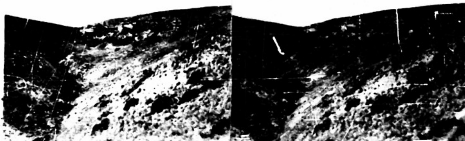
Ground Photos 33-A and 33-B. Stereopair of view to northwest to head of Blackfeet Gulch in Section 26, T. 22 N., R. 4 E., showing vertical rock cliffs. Old road on causeway descended into canyon from right. (See map, Figure 5-A, and Airphotos 4-A and 4-B)
