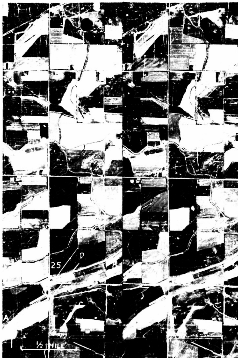
Airphotos 10-A and 10-B. Stereogram of area in Sections 17, 18, 19, 20, 29, 30, 31, and 32, T. 22 N., R. 2 W., Fairfield quadrangle, Montana. (See map, Figure 7)
