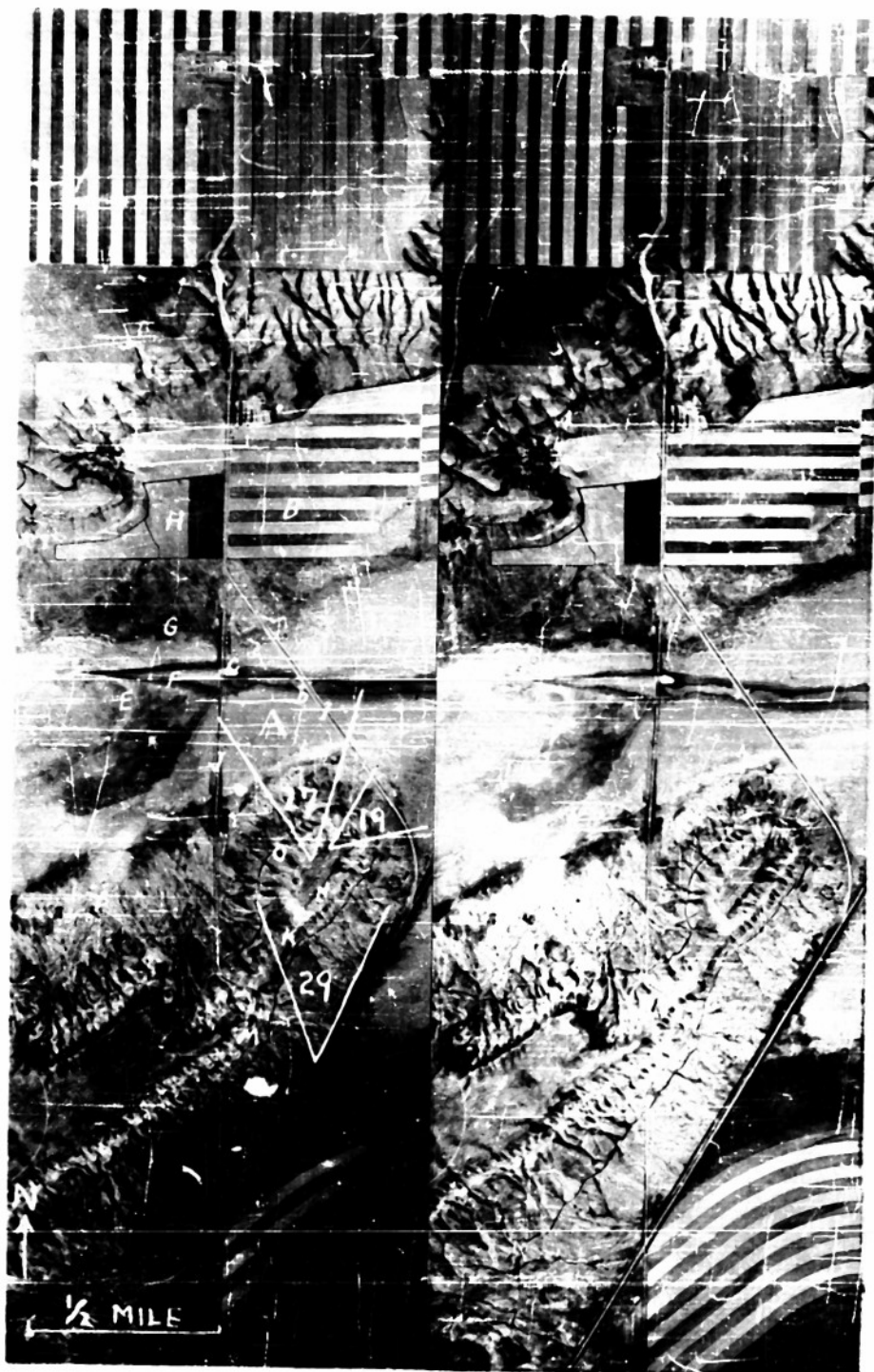
Airphotos 5-A and 5-B. Stereogram of area in Sections 28, 29, 32 and 33, T. 22 N., R. 4 E. and Sections 11, 5, 6, and 7, T. 21 N., R. 4 E., Portage quadrangle, Montana. (See map, Figure 5-B)
