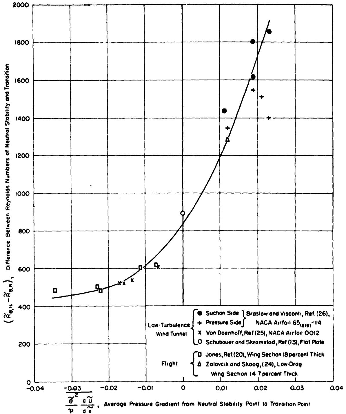
Figure 4 - Position of Self-Excited Transition as Function of Average Pressure Gradient
