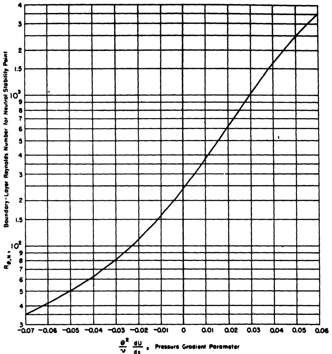
Figure 8 - Neutral Stability Point as Function of Pressure Gradient (Mangler, Ref. 21)
