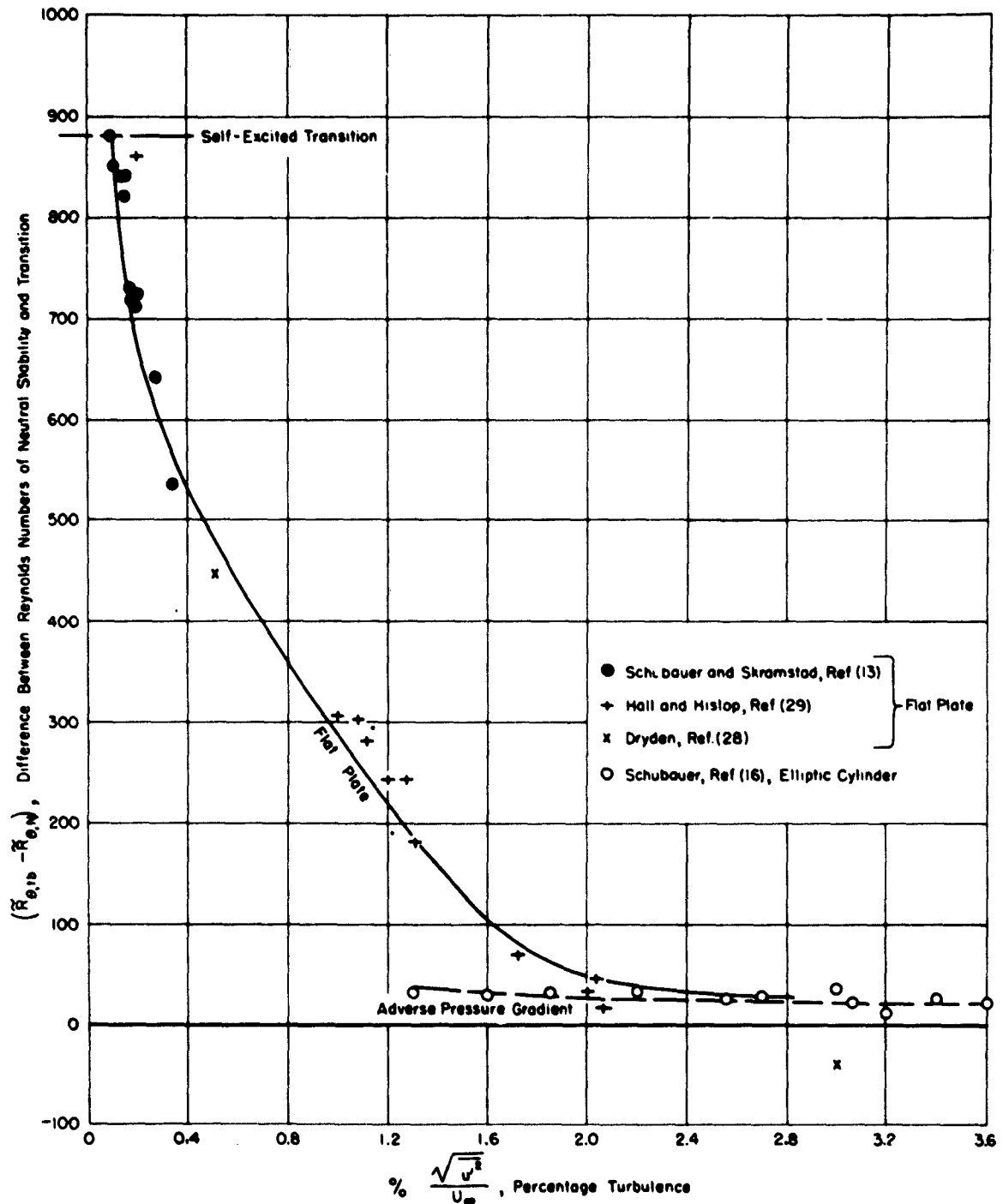
Figure 5 - Position of Transition in a Turbulent Stream
