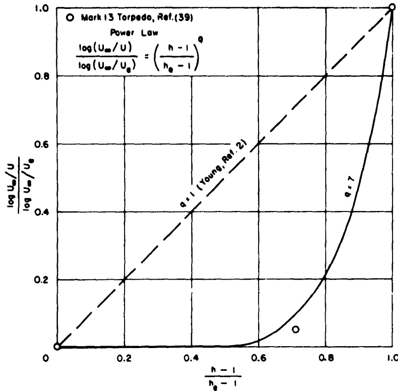
Figure 7 - Variation of Axisymmetric Shape Parameter h in Wake
