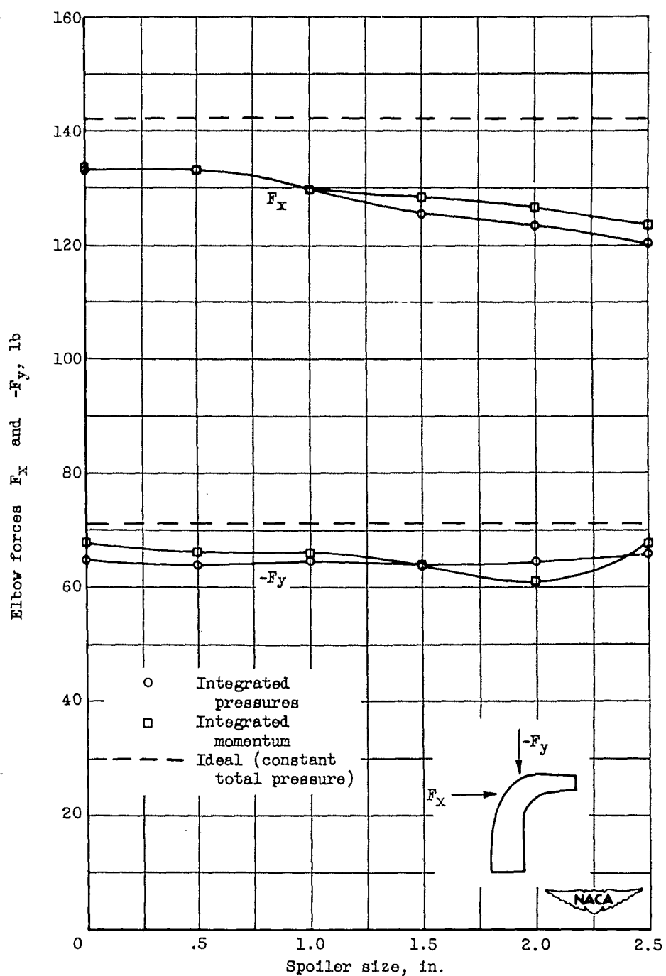
Figure 19. - Variation in x and y components of elbow force acting on fluid with spoiler size. Tank gage pressure ( p_T - p_A ), 20 inches of water.
