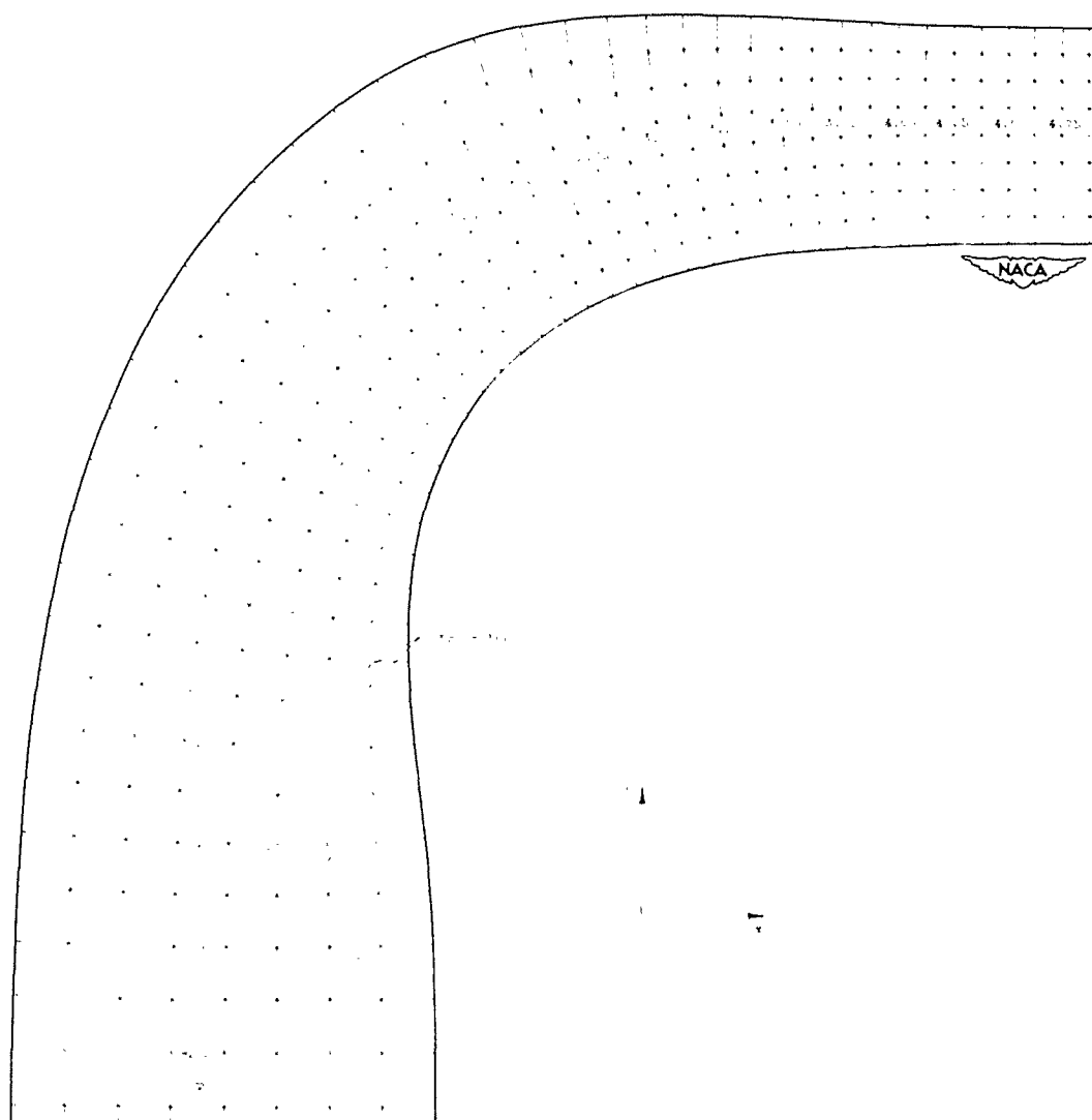
Figure 5. - Streamlines and velocity-potential lines in elbow plane. Incompressible flow; prescribed velocity given in table I.
