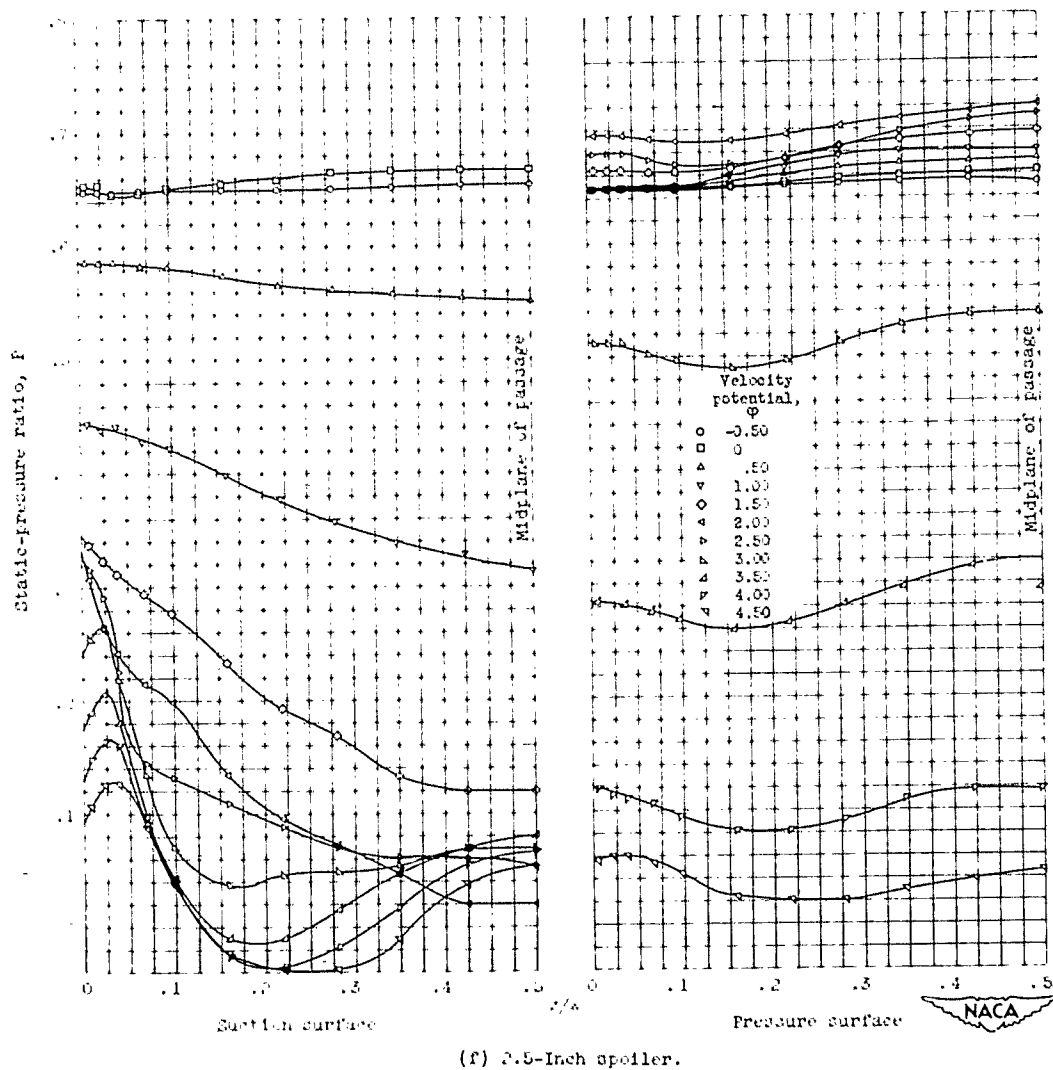
(f) 2.5-Inch spoiler. Figure 14. - Concluded. Spanwise distribution of static pressure on pressure and suction surfaces of elbow. Tank gage pressure ( P_T - P_a ) 20 inches of water.
