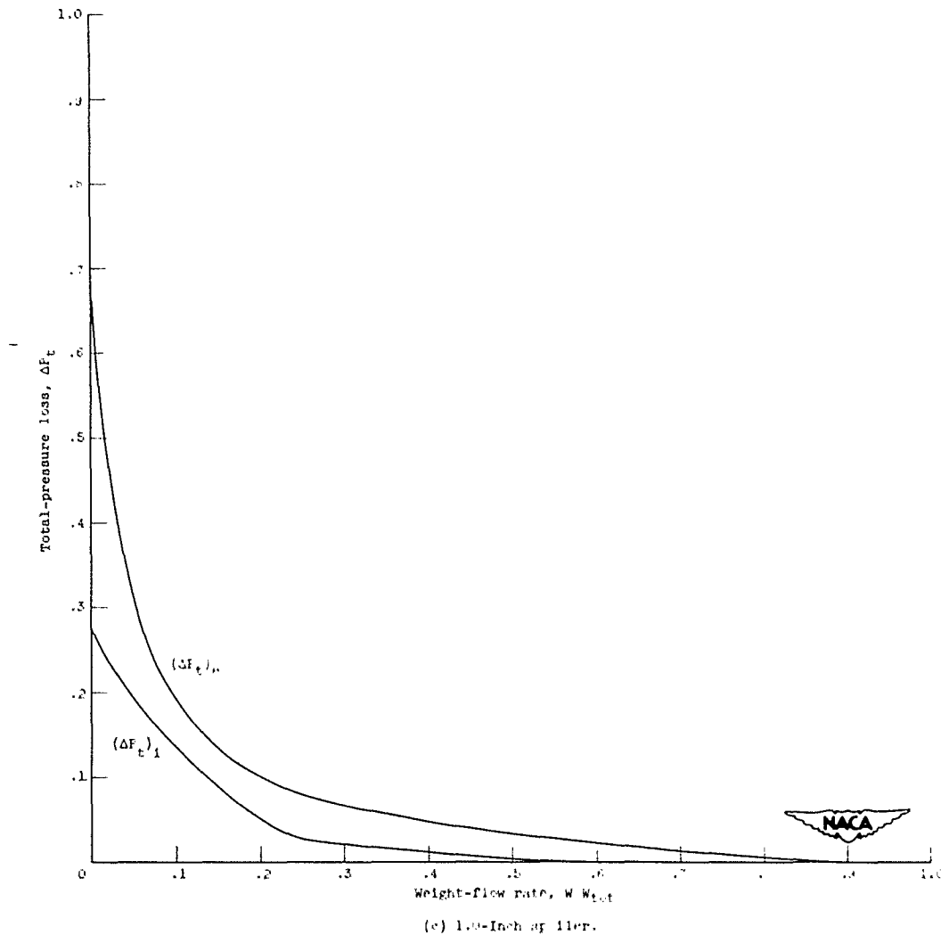
Figure 12. - Continued. Variation in total-pressure loss \Delta F_t at inlet and exit planes of elbow as a function of weight-flow ratio W/W_{tot} where, for each value of \Delta F_t , W/W_{tot} is percent of total weight-flow rate that has a total-pressure loss at least as high as \Delta F_t .
