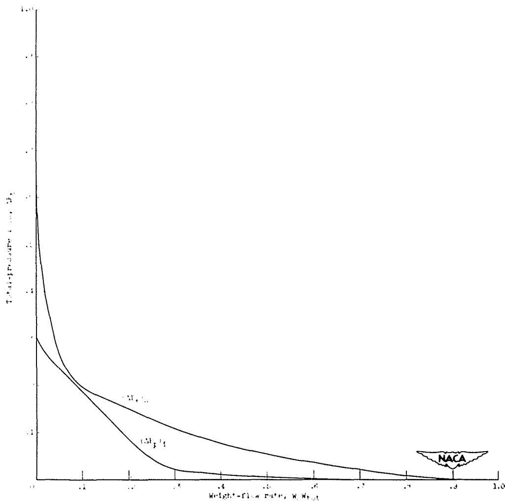
Figure 12. - Continued. Variation in total-pressure loss \Delta P_t at inlet and exit planes of elbow as a function of weight-flow ratio W/W_{tot} , where, for each value of \Delta P_t , W/W_{tot} is percent of total weight-flow rate that had a total-pressure loss at least as high as \Delta P_t .
