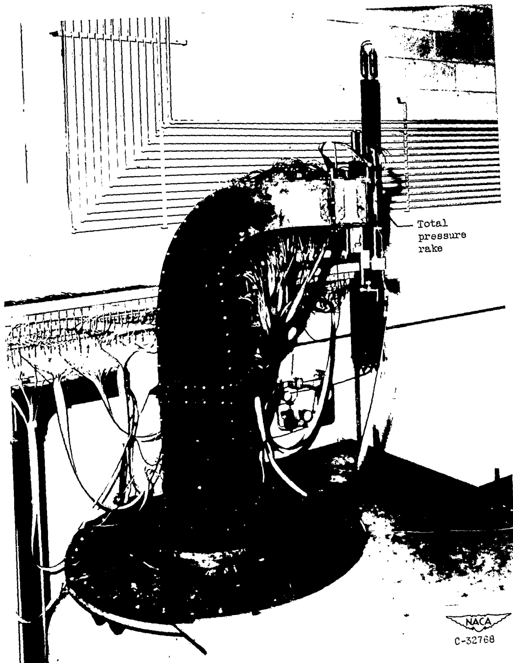
Figure 6. - Photograph of elbow installed on tank.
