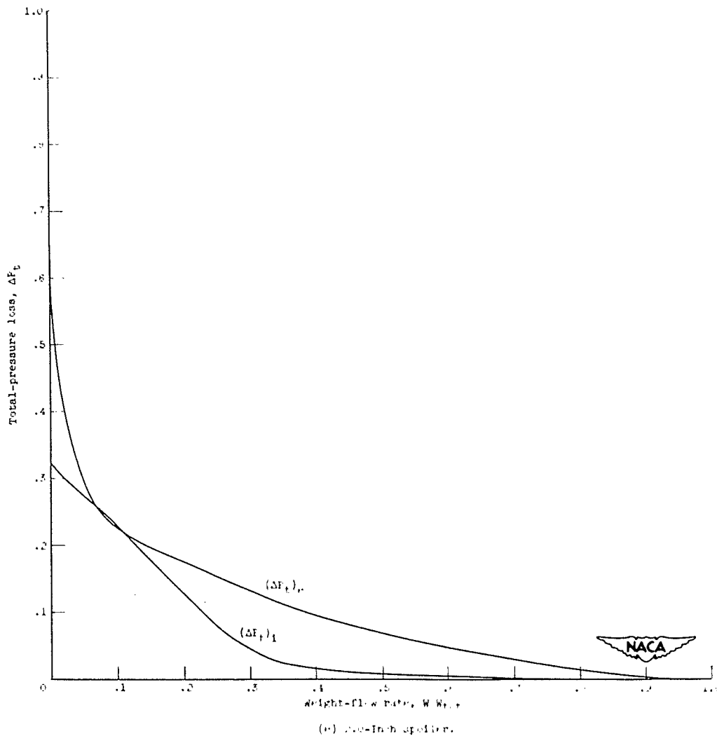
Figure 13. - Continued. Variation in total-pressure loss, \Delta P_t , at inlet and exit planes of airfoil as a function of weight-flow ratio W/W_{t,0} , where, for each value of \Delta P_t , W/W_{t,0} is percent of total weight-flow rate that has a total-pressure loss at least as high as \Delta P_t .
