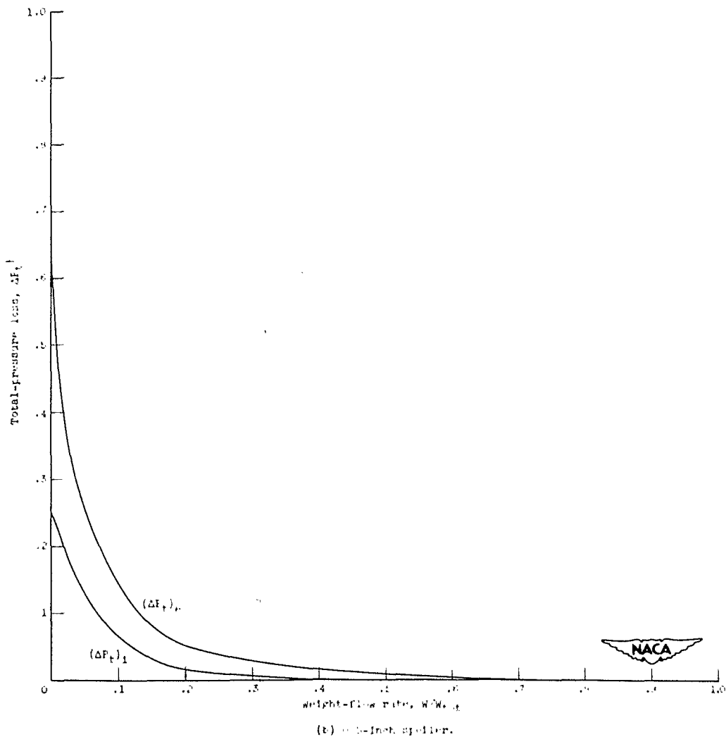
Figure 12. - Continued. Variation in total-pressure loss \Delta P_t at inlet and exit planes of elbow as a function of weight-flow ratio W/W_{tot} where, for each value of \Delta P_t , W/W_{tot} is percent of total weight-flow rate that has a total-pressure loss at least as high as \Delta P_t .
