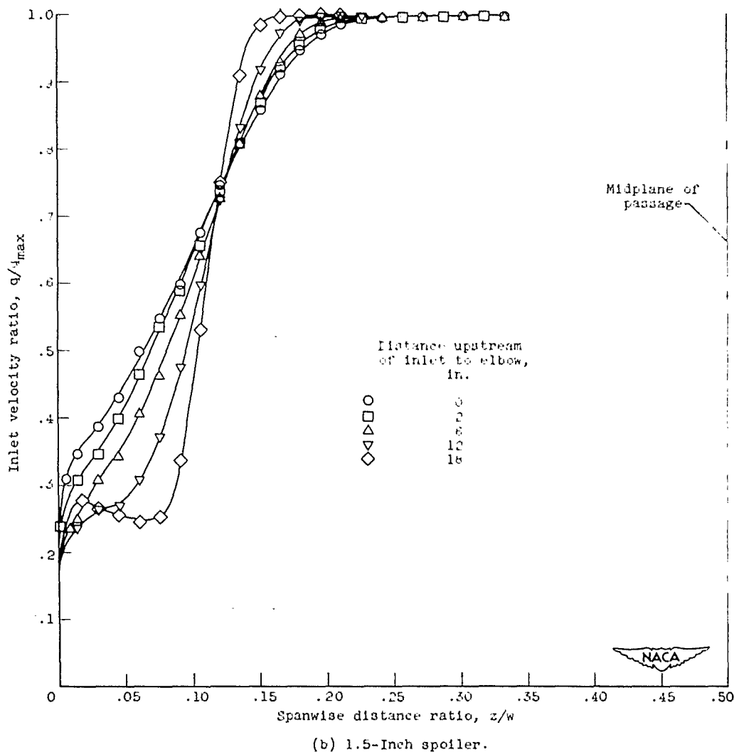
Figure 4. - Continued. Velocity profiles on plane walls of tunnel at center line for various distances upstream of inlet to elbow. Tank gage pressure ( p_T - p_a ), 20 inches of water.
