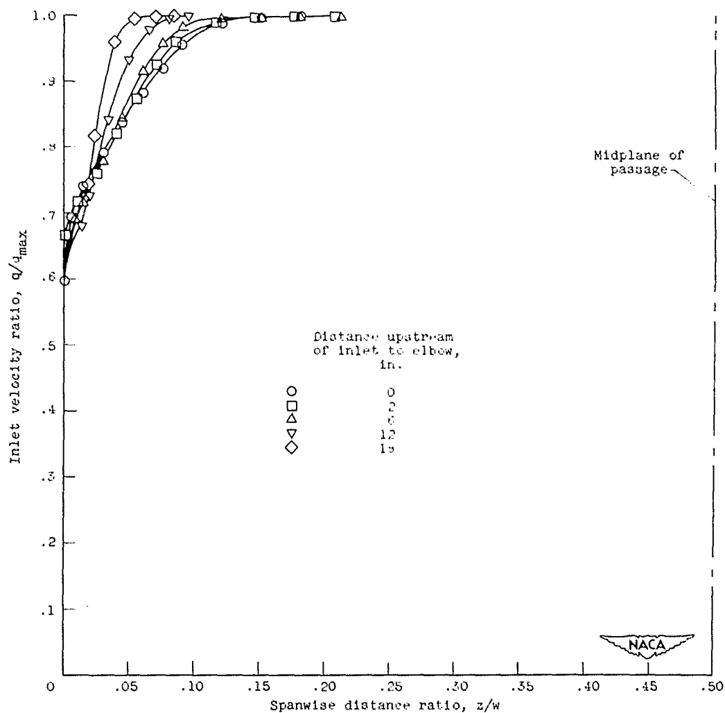
(a) 0.5-Inch spoiler.
