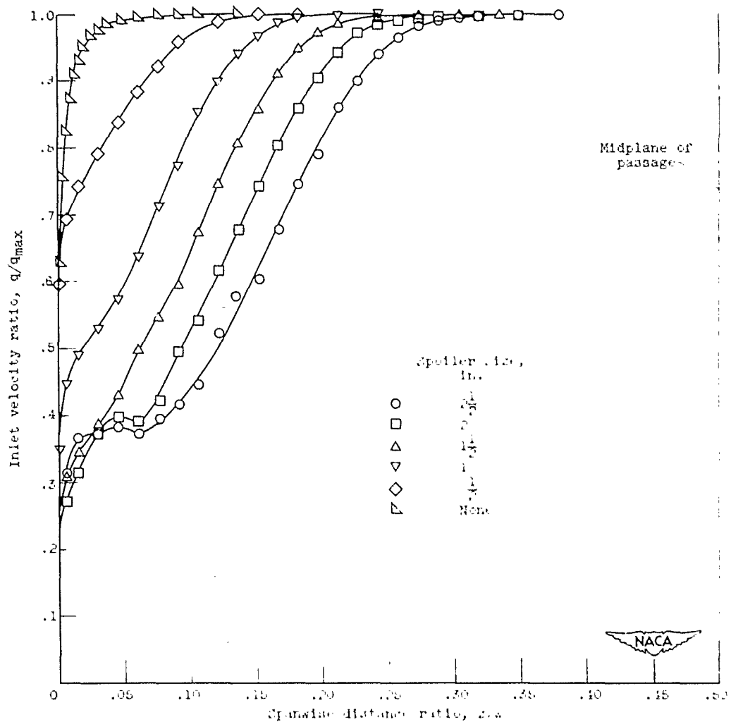
Figure 3. - Inlet velocity profiles on plane walls of elbow at center line for various spoiler sizes. Tank gage pressure ( P_T - P_D ), 30 inches of water.
