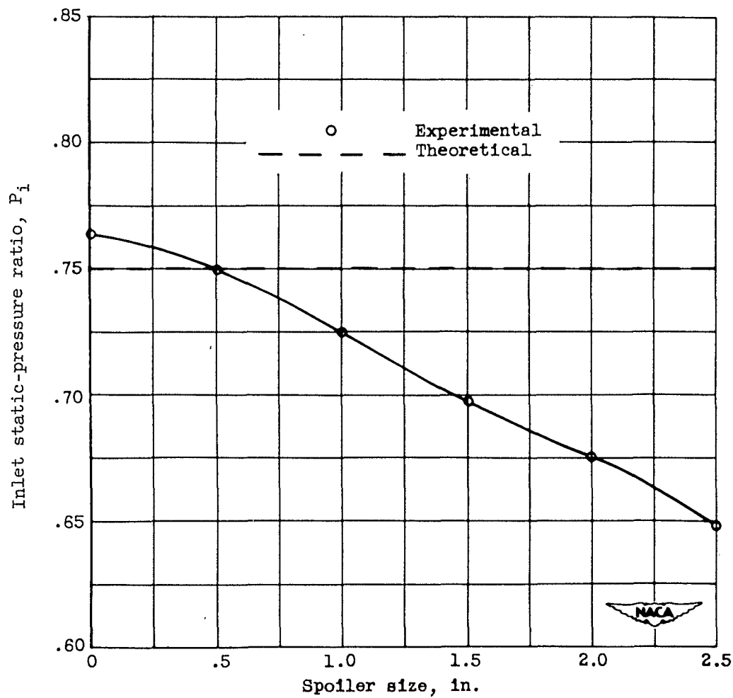
Figure 17. - Variation in inlet static pressure with spoiler size. Tank gage pressure ( p_T - p_a ), 20 inches of water.
