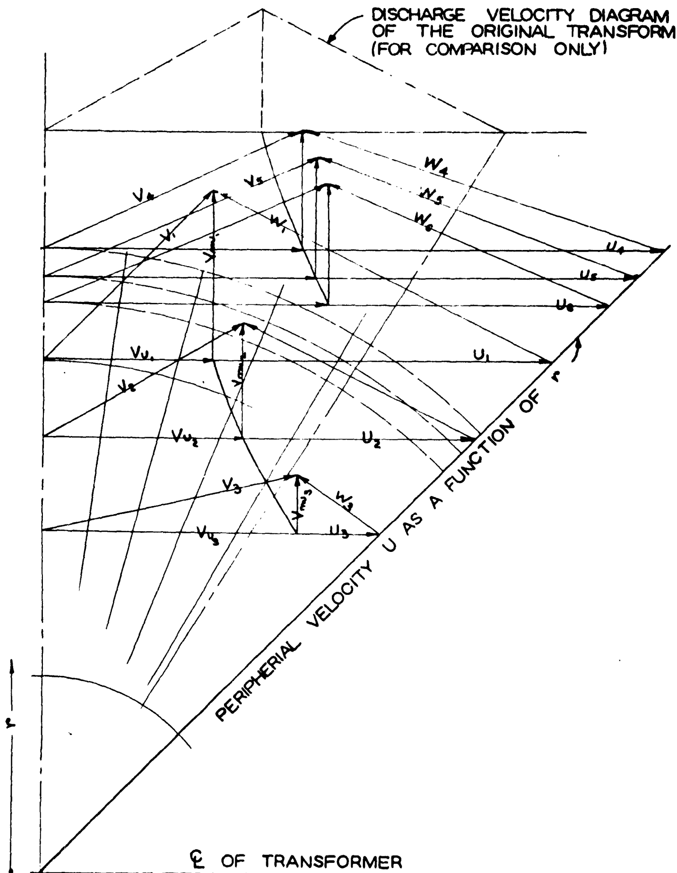
Velocity Diagrams of Primary Runner for a Transmission Ratio of 7.4 to 1
