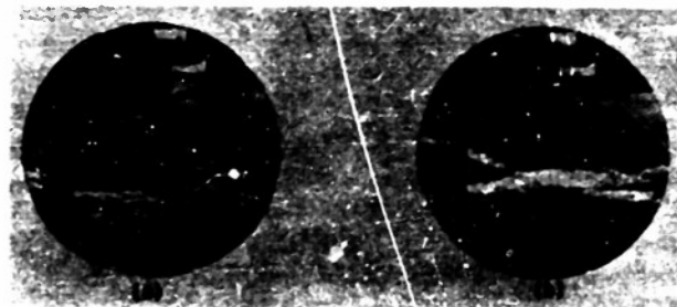
FIG. 11. Schlieren photographs of jet in test section before complete starting of tunnel; P_0 = 10 atm., T_0 = 25^\circ\text{C} . (a) P/P_0 = 60.8 and (b) P/P_0 = 62.8 . (Starting pressure ratio P/P_0 = 64.4 ; M' = 7.2 .)
