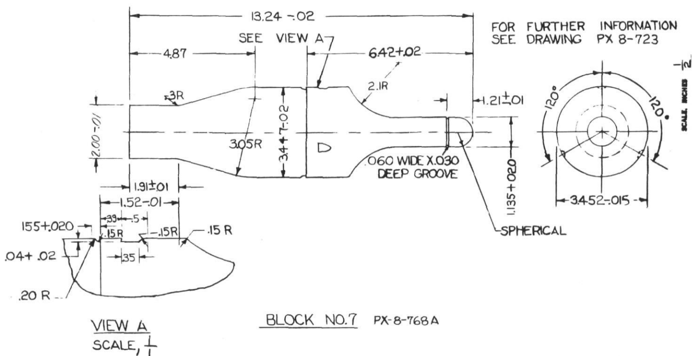
Figure XV—Block No. 7.
