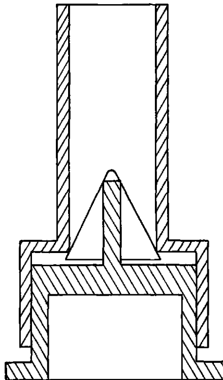
Figure 6—C.I.T. Mold.
