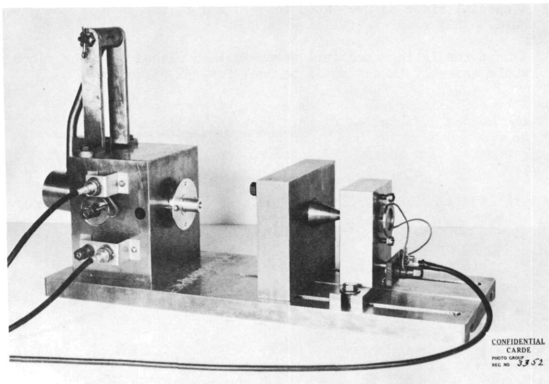
Figure 5—Test Fixture.
