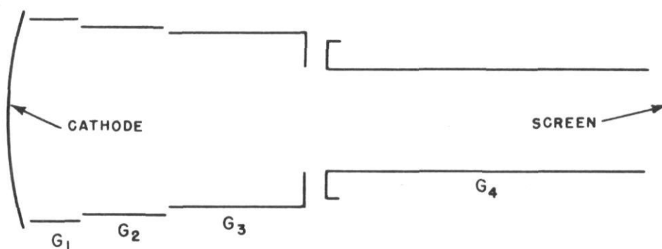
Figure 1—1P25A Image converter tube.
