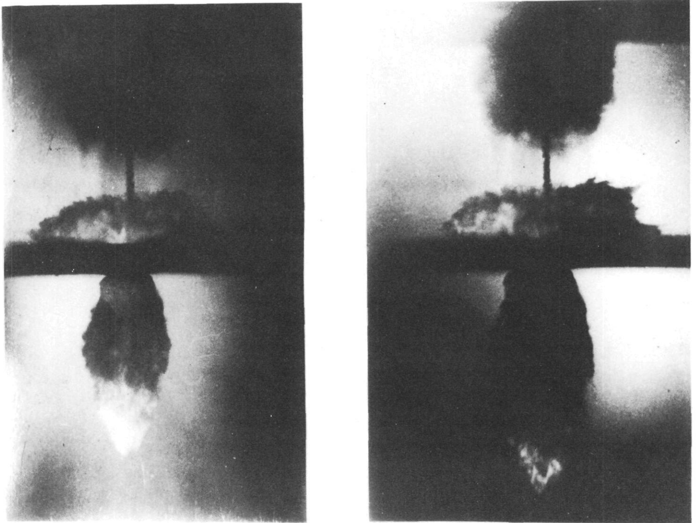
Figure 19—Two successive pictures of a jet penetrating \frac{1}{2} inch steel plate, taken with two Kerr cell cameras.
