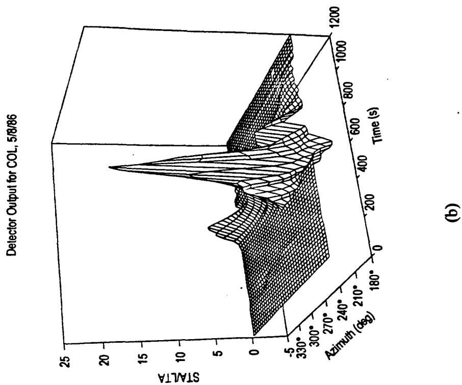
Figure 1. (a) Vertical, radial and transverse records from station COL of an M_S 5.4 earthquake in the Aleutian Islands on May 8, 1986, at a distance of 20^\circ and a backazimuth of 241^\circ . (b) Output of the detection algorithm for the signals shown in (a).
