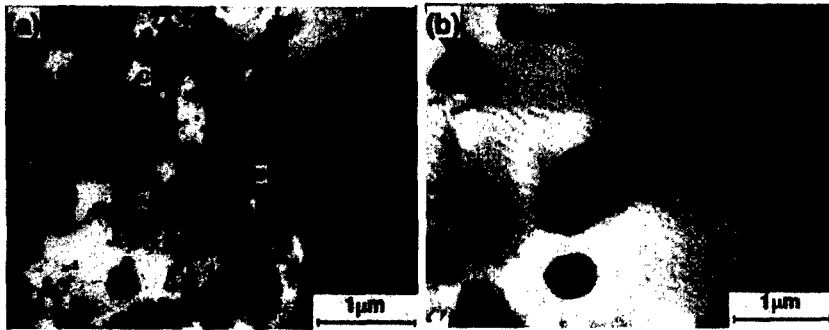
Fig.6 TEM micrographs for ECAP samples aged for 100 hours at (a) 373 K and (b) 473 K.
