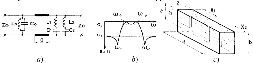
Fig. 2. A passing cascade section at the replacement of one passing circuit by a pair of rejection circuits (a), its frequency response (b) and design (c)
