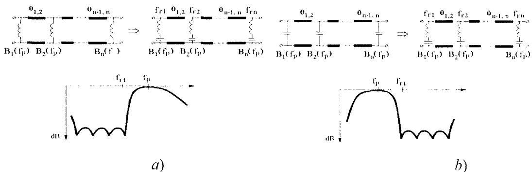
Fig. 3. Transformation of a polynomial filter into the filter with poles: a) in the bottom stopband (quasi-high-pass filter); b) in the top stopband (quasi-low-pass filter)
