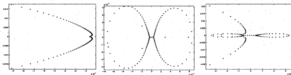
FIG. 1. Eigenspectra where b(t) has no change of sign on [0, 1] (left), where b(t) has a change of sign on [0, 1] and \int_0^1 b(s) ds = 0 (centre), and where b(t) has a change of sign on [0, 1] and \int_0^1 b(s) ds \neq 0 (right).
