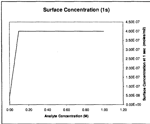
Figure 3. Analyte concentration vs. surface concentration at 1 second.
