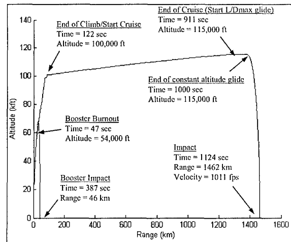
Figure 8: Maximum Range Mission Trajectory Profile
