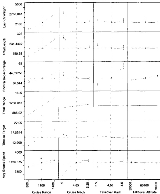
Figure 4: Parametric Dynamic Design Space Exploration Environment
