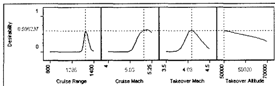
Figure 7: Desirability Curves for the Design Variables
