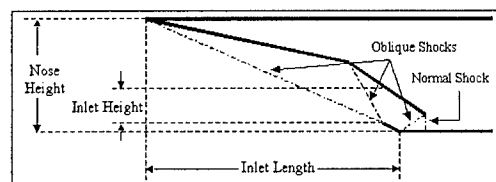
Figure 2: Inlet Analysis Configuration
