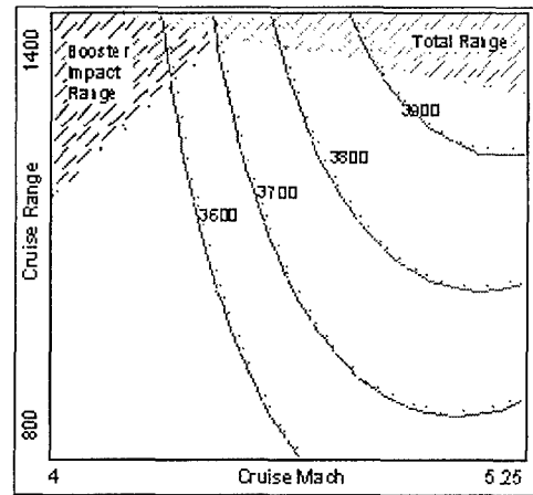
Figure 6: Cruise Segment Dynamic Tradeoff Environment
