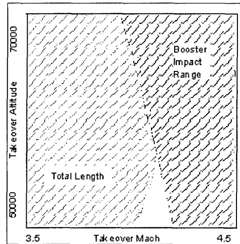
Figure 5: Booster/Ramjet Takeover Dynamic Tradeoff Environment
