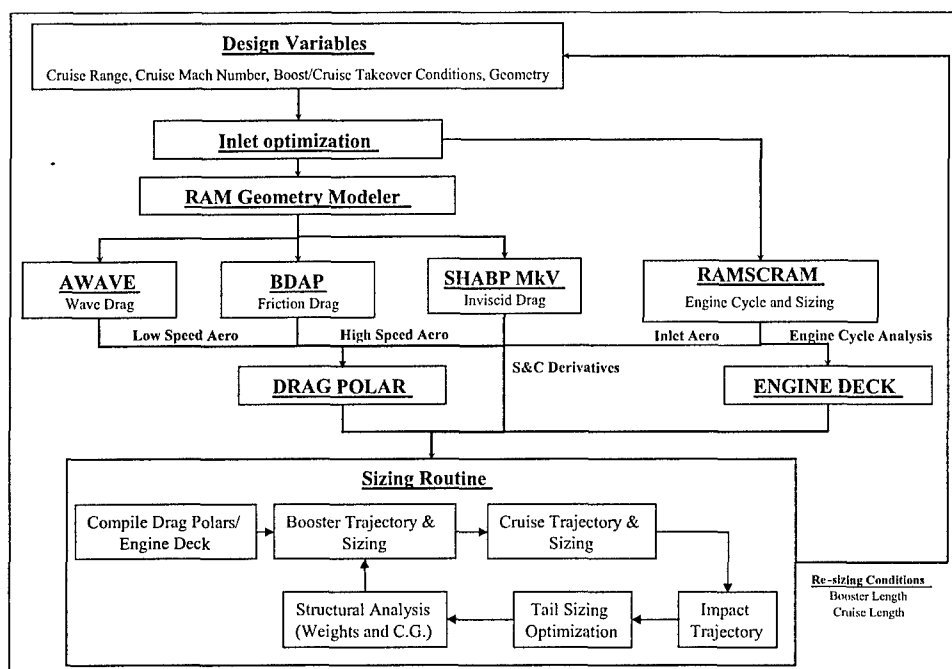
Figure 3: The Integrated Sizing &amp; Synthesis Environment
