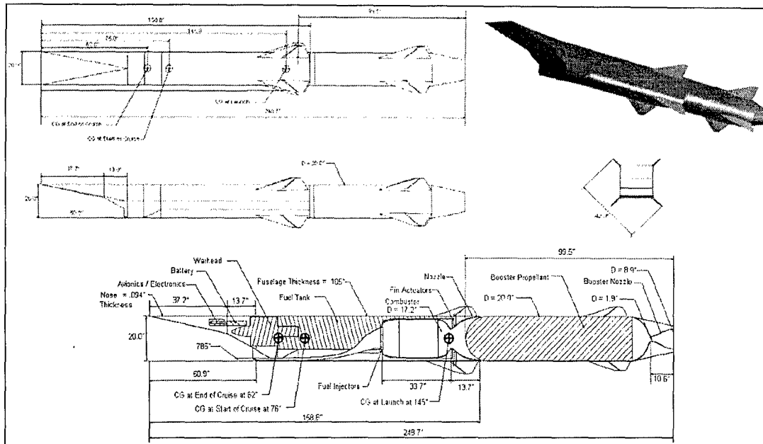
Figure 9: Hypersonic Cruise Missile Layout
