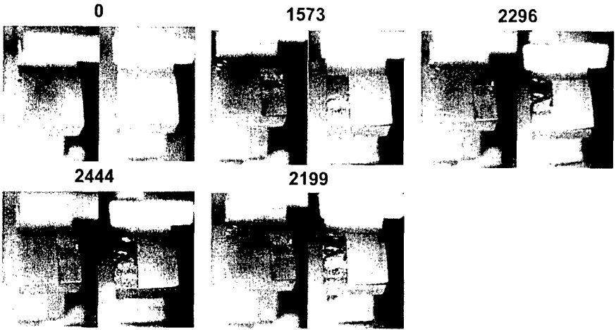
Figure 5.—Damage progression of driver/driven tooth 11 for experiment 3.
