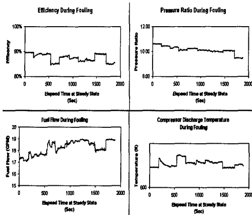
Figure 4 – Parameter Deviation at Full Load (LM2500 test)
