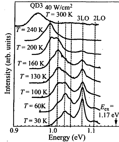
Fig. 3. Temperature dependence of the resonant PL spectra for the structure QD3.
