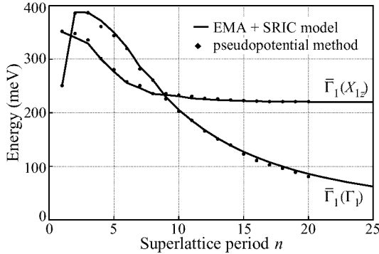
Fig. 1. Energy of the two lowest conduction states of (GaAs) n /(AlAs) n (001) SL.
