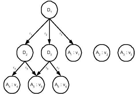
Figure 2. Basic set-covering model for diagnosis D
