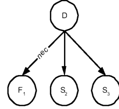
Figure 6. Necessary Covering relation for a diagnosis D .
