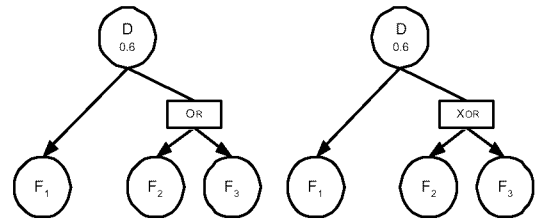
Figure 4. OR-/XOR-covering relations.
