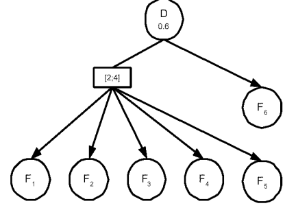
Figure 5. A [MIN, MAX]-covering relation.
