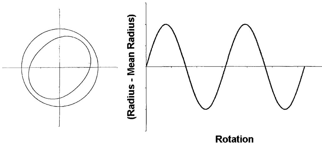
FIGURE 9. Out-of-Roundness.
