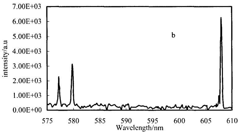
(a) N_2:Cl_2 = 0:106, 30\text{Torr} (b) N_2:Cl_2 = 117:110, 18\text{Torr}
