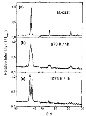
Figure 10. Effect of annealing on X-ray patterns of \text{Co}_{29}\text{Ni}_{25}\text{Mn}_1\text{Cu}_{45} microwire
