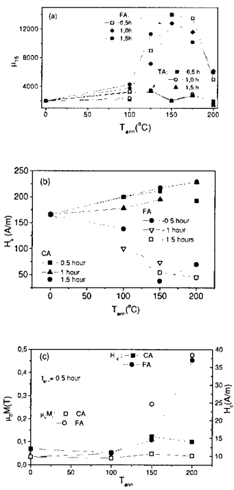
Figure 3. Effect of annealing on magnetic properties of \text{Co}_{69}\text{Mn}_6\text{Si}_{10}\text{B}_{15} microwires: initial magnetic permeability, \mu_{15} (a), anisotropy field, H_k (b), coercivity and remanent magnetization (c)
