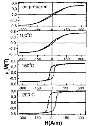
Figure 2. Effect of magnetic field annealing (FA) on hysteresis loops of (\text{Co}_{0.92}\text{Mn}_{0.8})_{75}\text{Si}_{10}\text{B}_{15} microwire at different annealing temperatures.
