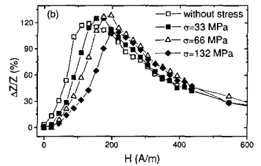
Figure 6. Effect of the frequency, f , (a) and applied stresses (b) on \Delta Z/Z ratio of \text{Co}_{68.5}\text{Mn}_{6.5}\text{Si}_{10}\text{B}_{15} amorphous microwire
