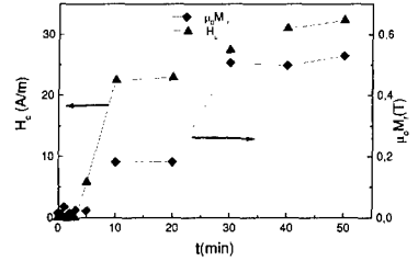
Figure 5. Effect of chemical etching on the magnetic parameters of the \text{Co}_{68}\text{Mn}_7\text{Si}_{10}\text{B}_{15} amorphous microwire.
