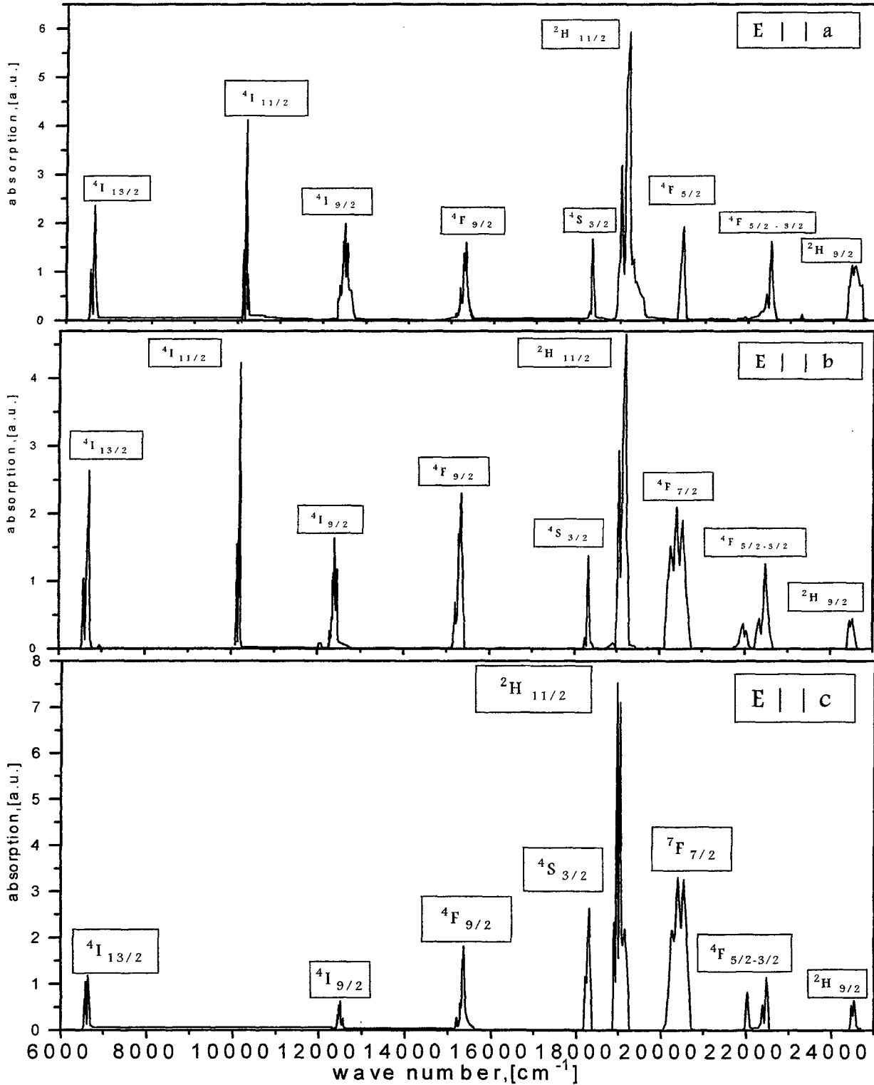
Fig1. The main optical absorption spectra of \text{KEr}(\text{WO}_4)_2 are connected with 4f^{11} electron configuration of \text{Er}^{3+} ions. Ground state multiplet for \text{Er}^{3+} ions is ^4I_{15/2} . The next multiplets are ^4I_{13/2} , ^4I_{11/2} , ^4I_{9/2} , ^4F_{9/2} , ^4S_{3/2} , ^2H_{11/2} , ^4F_{5/2} , ^4F_{3/2} , ^2F_{5/2} , ^2H_{9/2} . Figure presents optical transitions to all above excited multiplets at temperature 1.1 K.
