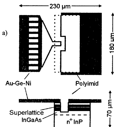
Fig. 1: Planar superlattice device SLED (a) mounted in waveguide structure (b).
