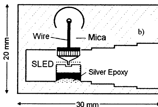
Fig. 1: Planar superlattice device SLED (a) mounted in waveguide structure (b).
