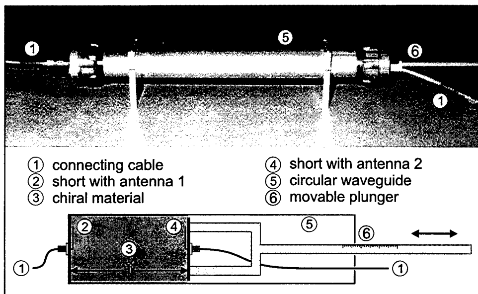
Fig. 3 Experimental setup.
