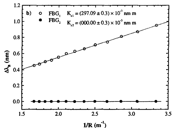
Fig. 2 Response of smart sensor plate to: a) Temperature; b) Inverse curvature radius ( 1/R ).
