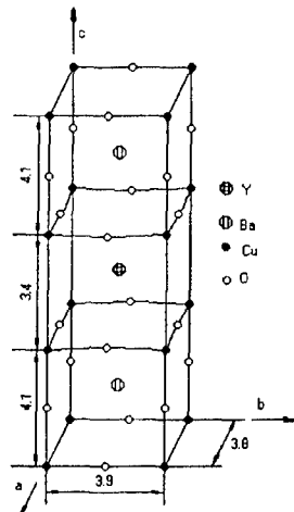
Fig. 1. Structural lattice of Y_1Ba_2Cu_3O_7 .
