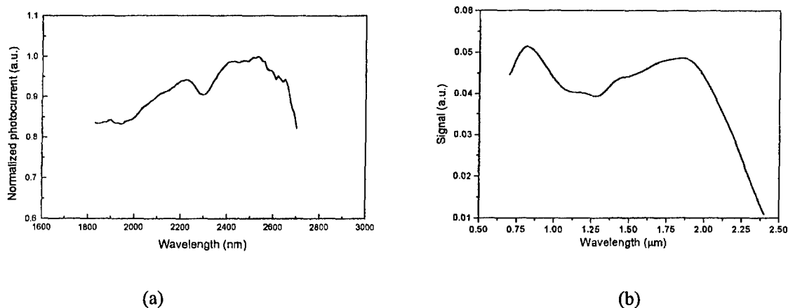
Fig. 4. Spectral distribution of photoconductive signal normalized to the incident power for PbS films: (a) "standard" film measured in modulated light; (b) "nanocrystalline" film measured in permanent light.
