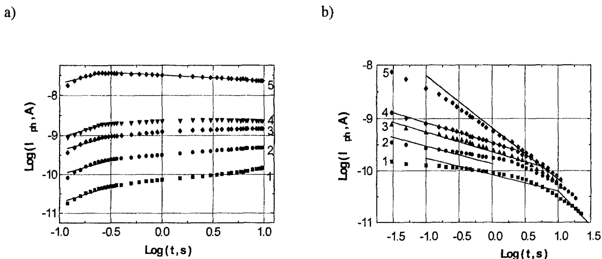
Fig.4. Double-logarithmic plot of photocurrent rise (a) and decay (b) in the \text{As}_{50}\text{Se}_{50} film at various light intensities F, \text{cm}^{-2}\cdot\text{s}^{-1} : 1 - 5.3 \cdot 10^{11} , 2 - 2.4 \cdot 10^{12} , 3 - 6.6 \cdot 10^{12} , 4 - 1.5 \cdot 10^{13} , 5 - 6.5 \cdot 10^{14} . Straight-line portions are calculated with \alpha = 0.67 (see text for details).
