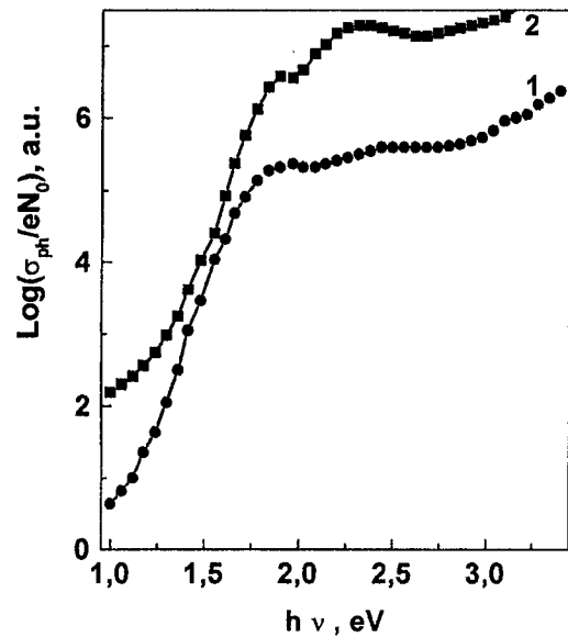
Fig. 2. The spectral dependence of the photoconductivity of laser (1) and thermal (2) deposited As_{40}Se_{60} (a) and As_{50}Se_{50} (b) thin films. The positive voltage is applied to the top illuminated electrode.
