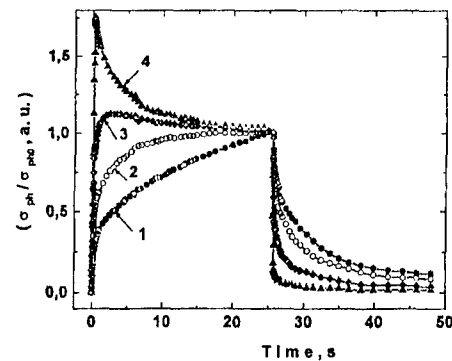
Fig. 3b. Photoconductivity relaxation curves in Au- As_{50}Se_{50} -Al thin films ( L=5.87 \mu\text{m} ) at T=290 \text{ K} . Light intensity F , %: 1 - 0.008; 2 - 0.3; 3 - 2.2; 4 - 100. F_0=6.5 \cdot 10^{14} \text{ cm}^{-2} \cdot \text{s}^{-1} , \lambda=0.63 \mu\text{m} .
