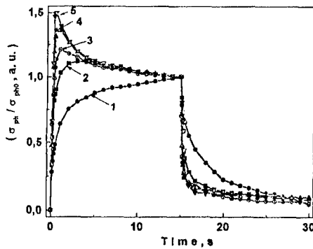
Fig. 3a. Photoconductivity relaxation curves in Au- As_{40}Se_{60} -Al thin films ( L=9.7 \mu\text{m} ) at T=290 \text{ K} . Light intensity F , %: 1-0.008; 2-2.2; 3-13; 4-37; 5-100. F_0=6.5 \cdot 10^{14} \text{ cm}^{-2} \cdot \text{s}^{-1} , \lambda=0.63 \mu\text{m} .
