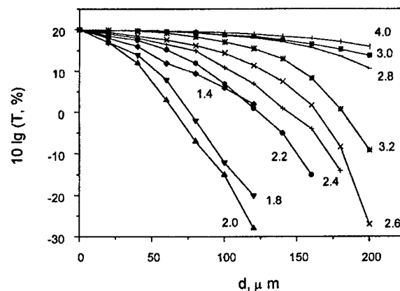
Fig. 2. Optical transmission characteristics vs. displacement amplitude for different microbend periods. = 1.4-4.0 m. The light source was a He-Ne laser coupled through a 90x microobjective.
