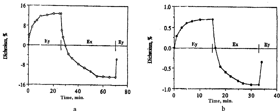
Fig. 3. Kinetics of dichroism generation and reorientation in as-prepared (a) and annealed at 210 °C (b) Ge 32 As 8 S 60 glassy film, measured by 515 nm probing laser beam.
