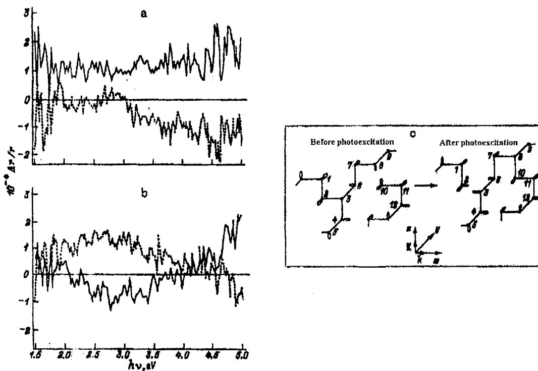
Fig. 6. Photoinduced reflectance anisotropy (solid lines) and its reorientation (dotted lines) in an \text{As}_2\text{S}_3 bulk glass sample irradiated by the light of 1000 W Xe lamp (a) or \text{Ar}^+ ion laser (b) and schematic representation of photostructural changes induced by the above-band-gap light (c).
