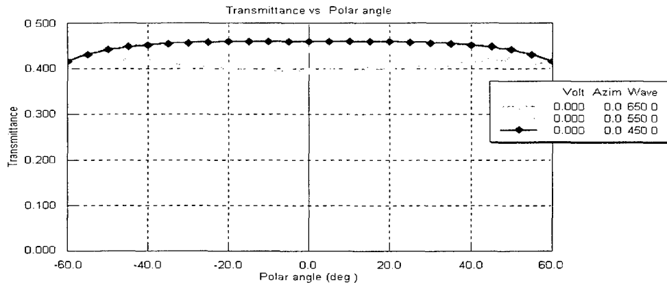
Figure 18. Normal 135/45 1-domain TN/LCD Red/Green/Blue transmission vs. viewing angle, and gray scale levels No. 1 and 8, for horizontal viewing zone with not films. LC: TL-203. 18(a).
