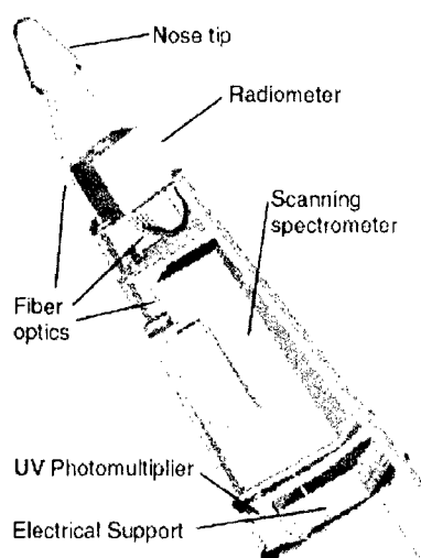
Figure 5. Rendering of CAD model showing fibers connecting the stagnation point and side looking directions from nose tip to appropriate instruments using long radii bends.
