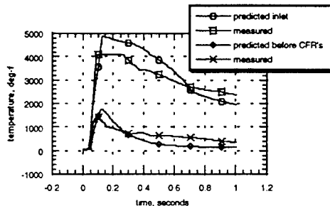
Fig 8 - JES-6 Dual CFR Model Predicted vs. Measured Inlet Temperatures, 25 mil Gap
