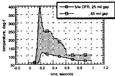
Fig 15 - FSM-9 Predicted Gas Temperatures in Assembly Gap Between CFRs
