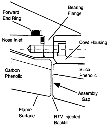
Fig 1- Current RSRM Nozzle Joint -2 Configuration
