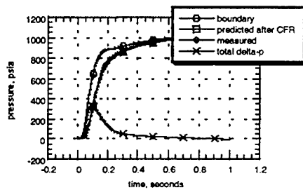
Fig 5 - JES-3 Single CFR Model Predicted vs. Measured Pressures, 25 mil Gap
