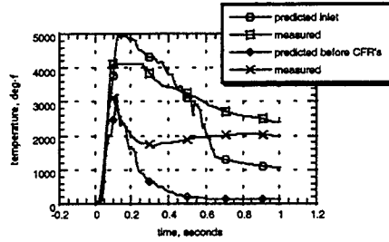
Fig 11 - JES-6 Predicted vs. Measured Temperatures Before CFRs in the Inlet Region, 65 mil Gap
