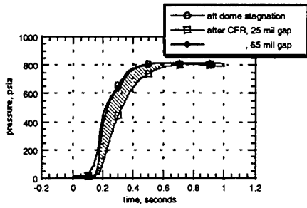
Fig 13 - FSM-9 Predicted Pressures
