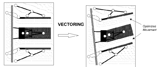
Fig. 14b.- Vectoring with hinged reaction bars
