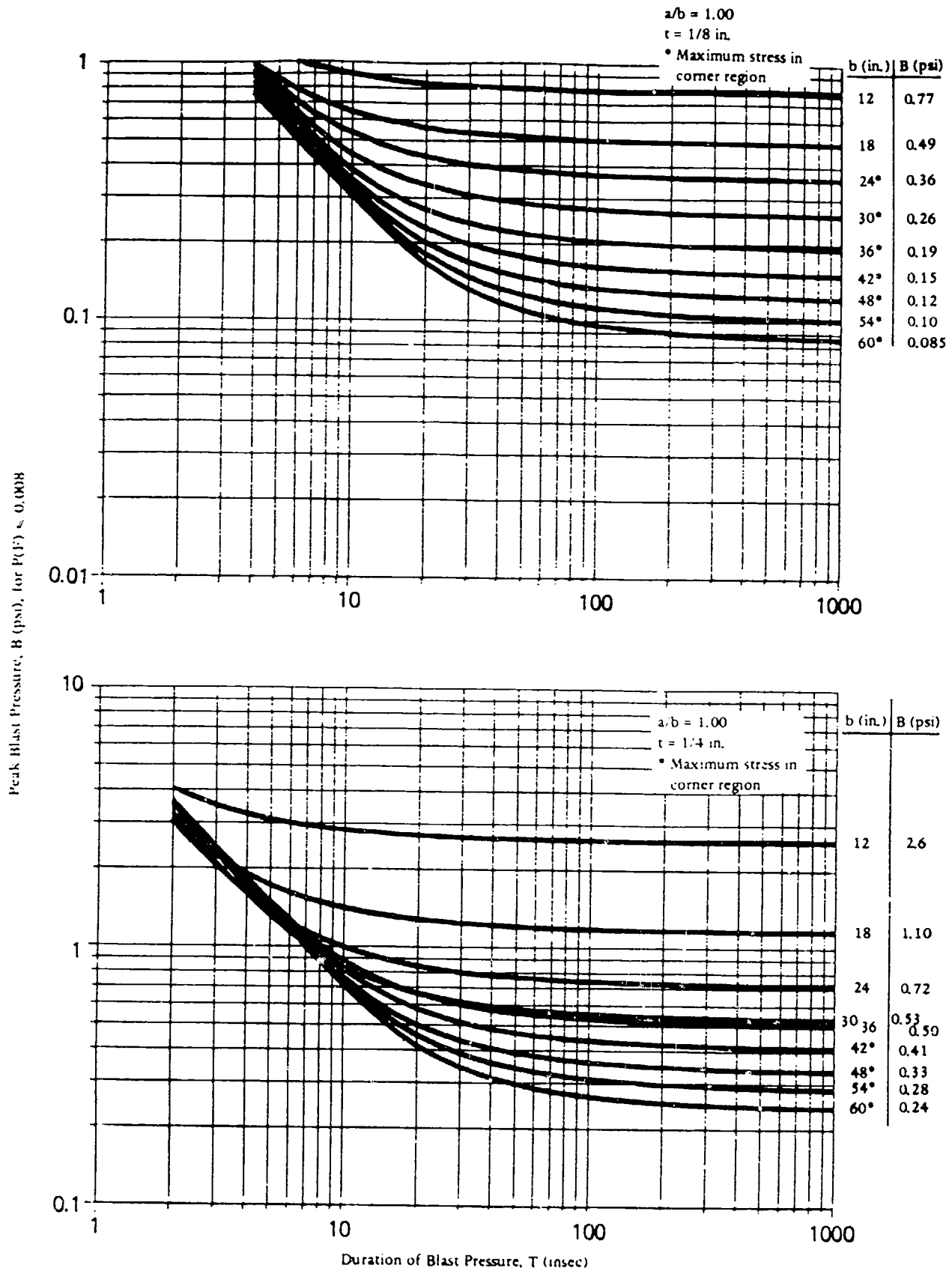
Figure 12. Peak blast pressure capacity for annealed glass panes: a/b = 1.00 , t = 1/8 and 1/4 in.
