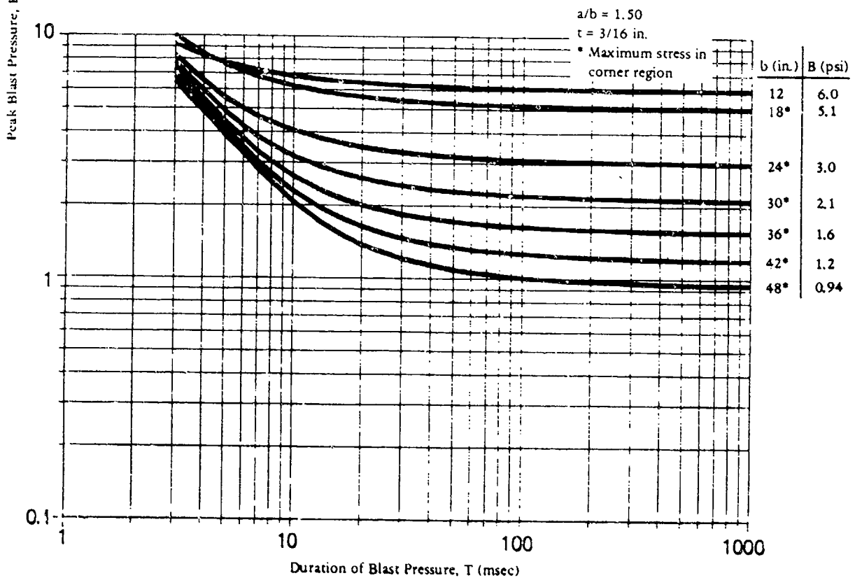
Figure 7. Peak blast pressure capacity for tempered glass panes: a/b = 1.50 , t = 1/4 and 3/16 in.
