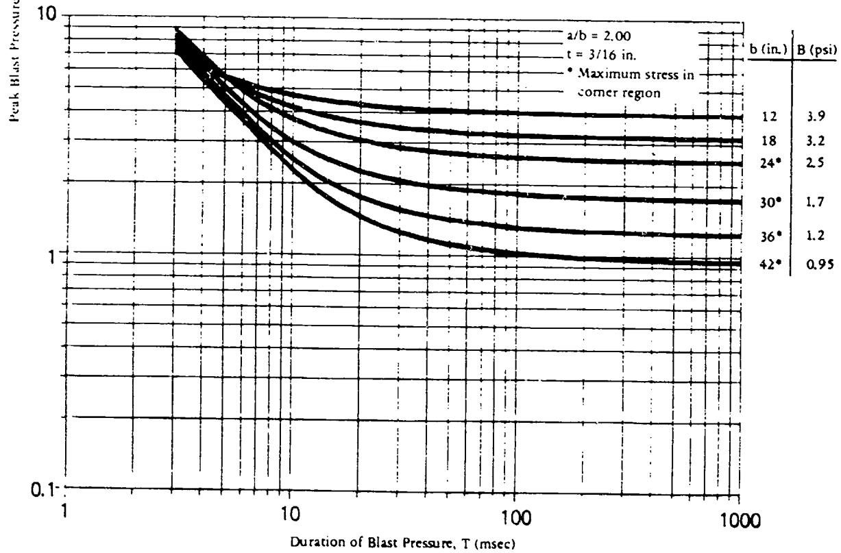
Figure 11. Peak blast pressure capacity for tempered glass panes: a/b = 2.00 , t = 1/4 and 3/16 in.
