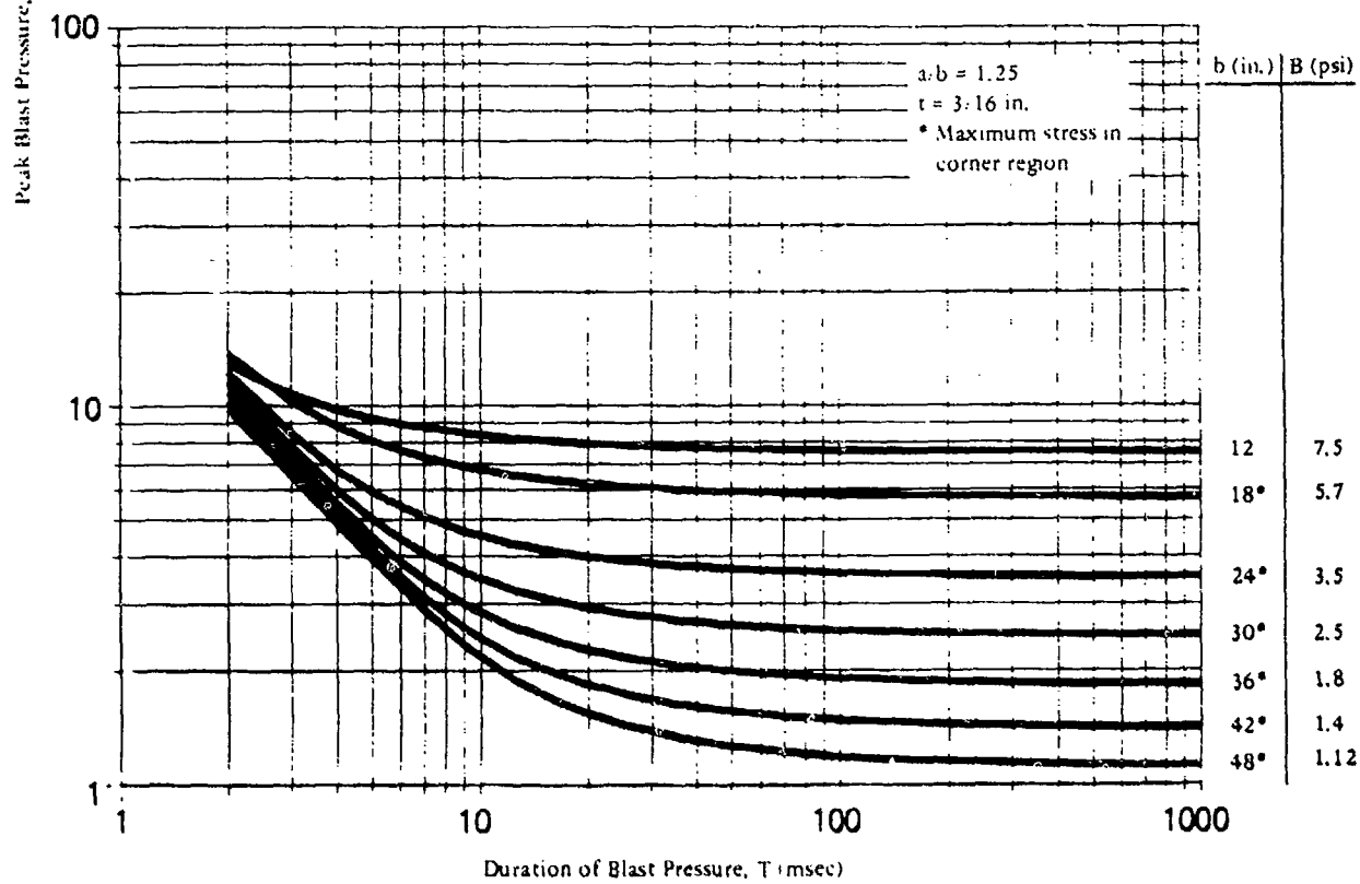
Figure 5. Peak blast pressure capacity for tempered glass panes: a/b = 1.25 , t = 1/4 and 3/16 in.
