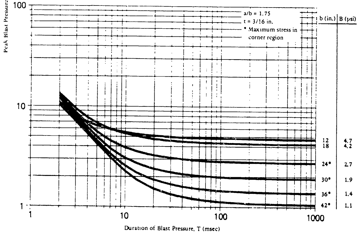
Figure 9. Peak blast pressure capacity for tempered glass panes: a/b = 1.75 , t = 1/4 and 3/16 in.
