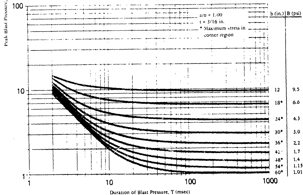
Figure 3. Peak blast pressure capacity for tempered glass panes: a/b = 1.00 , t = 1/4 and 3/16 in.
