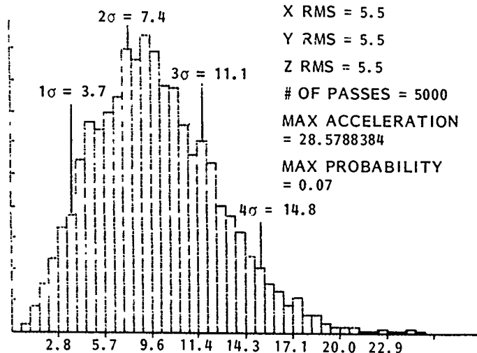
Figure 10. Vector Acceleration Probability Distribution
