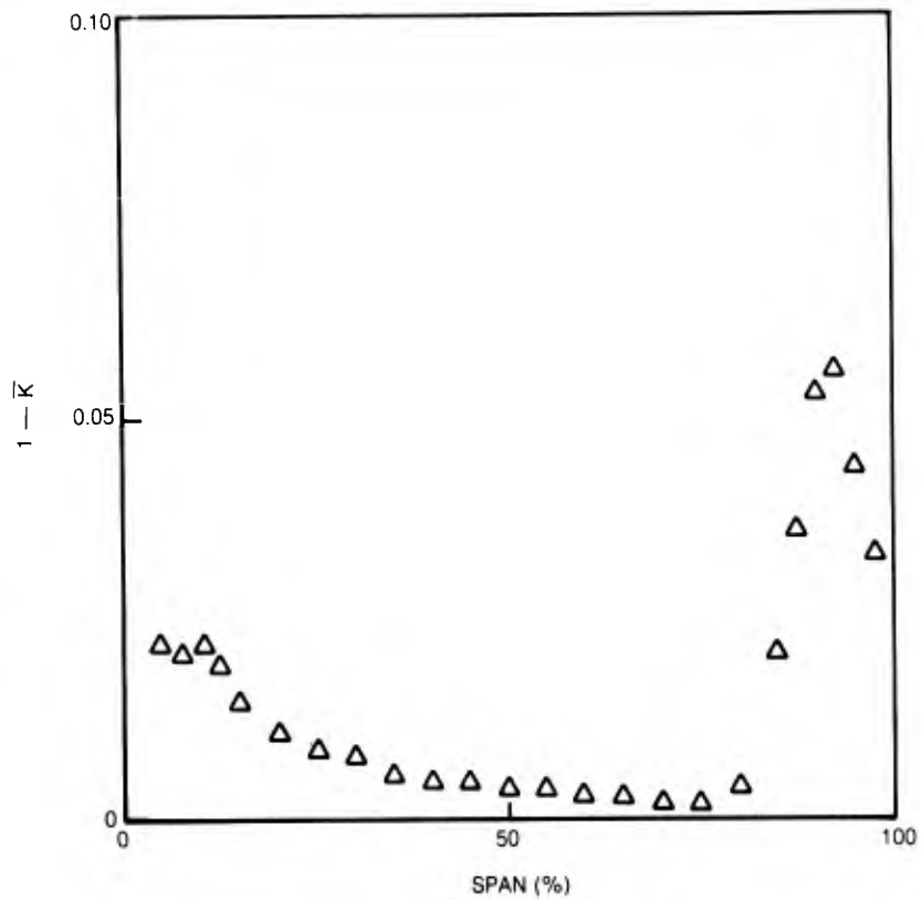
Figure 12 Two Stage Compressor, Second Stage Rotor, Blockage, \phi = 0.51
