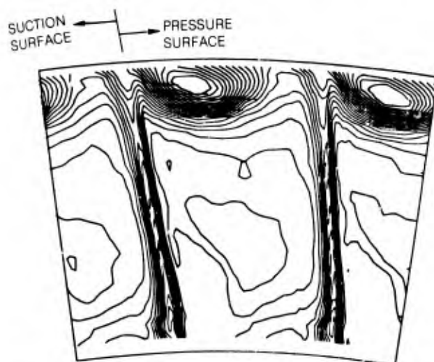
Figure 6 Two Stage Compressor, Second Stage Rotor, Rotary Total Pressure, \phi = 0.51 , 25% aft, 2.0 pitches, \Delta C_{PT} = 0.025
