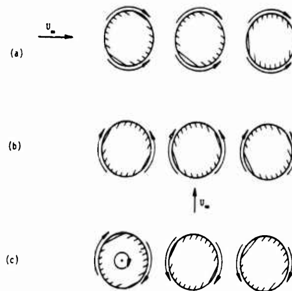
Fig. 5. Nonuniqueness of potential-flow solutions. (a) Noncirculatory flow with freestream at \alpha = 0^\circ . (b) Noncirculatory flow with freestream at \alpha = 90^\circ . (c) Circulatory flow with stagnant freestream.
