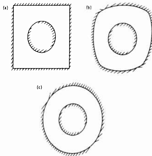
Fig. 10. Transformation to an annular region. (a) Original geometry. (b) Geometry after four corner-removing mappings. (c) Geometry after two circle mappings and two inversions.
